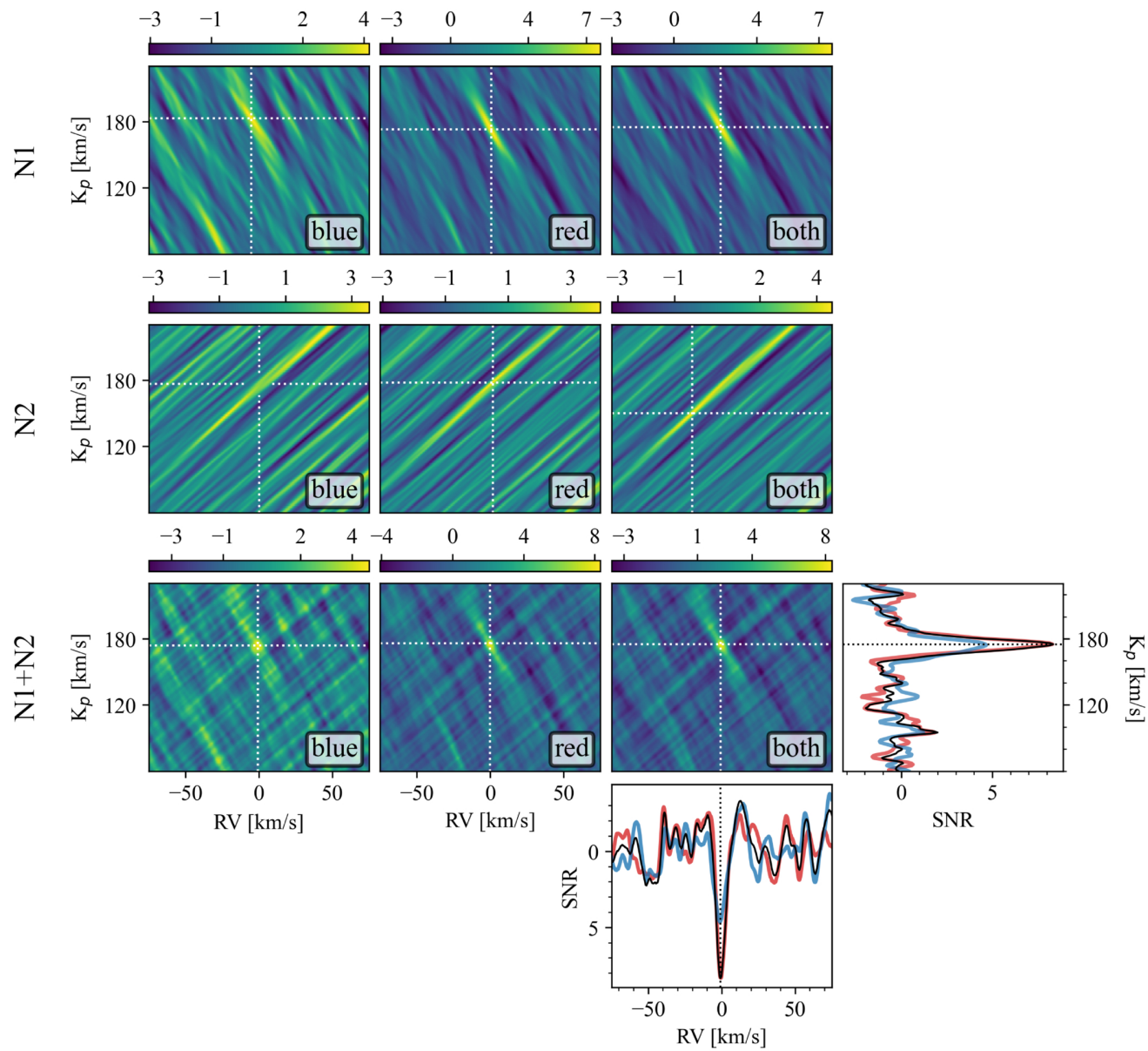
Figure 5. from Caitlin E. Bell et al 2026 Astron. J. 172 doi:10.3847/1538-3881/ae975e https://dx.doi.org/10.3847/1538-3881/ae975e © 2026. The Author(s). Published by the American Astronomical Society.
