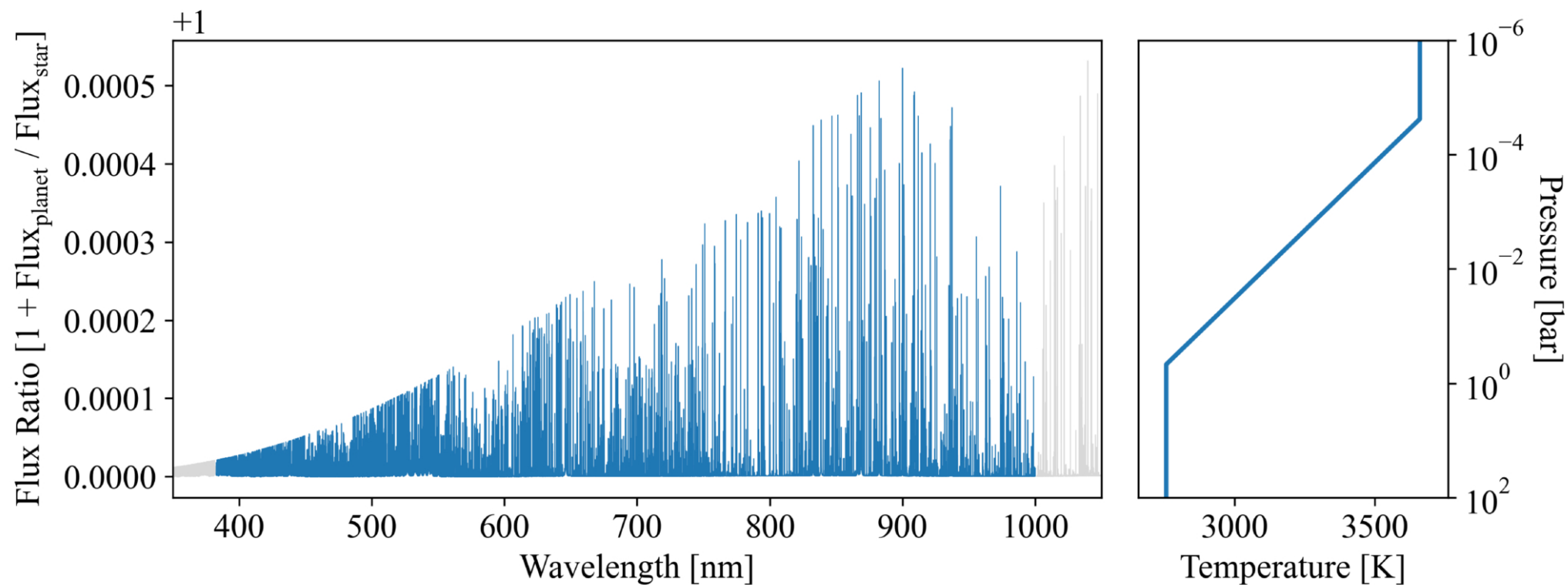
Figure 4. from Caitlin E. Bell et al 2026 Astron. J. 172 doi:10.3847/1538-3881/ae975e https://dx.doi.org/10.3847/1538-3881/ae975e © 2026. The Author(s). Published by the American Astronomical Society.
