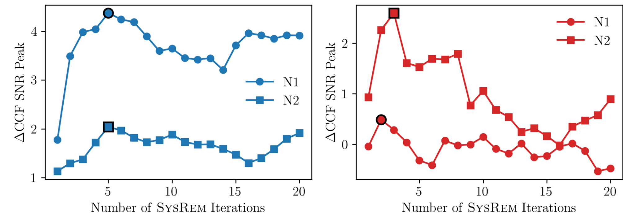
Figure 3. from Caitlin E. Bell et al 2026 Astron. J. 172 doi:10.3847/1538-3881/ae975e https://dx.doi.org/10.3847/1538-3881/ae975e © 2026. The Author(s). Published by the American Astronomical Society.
