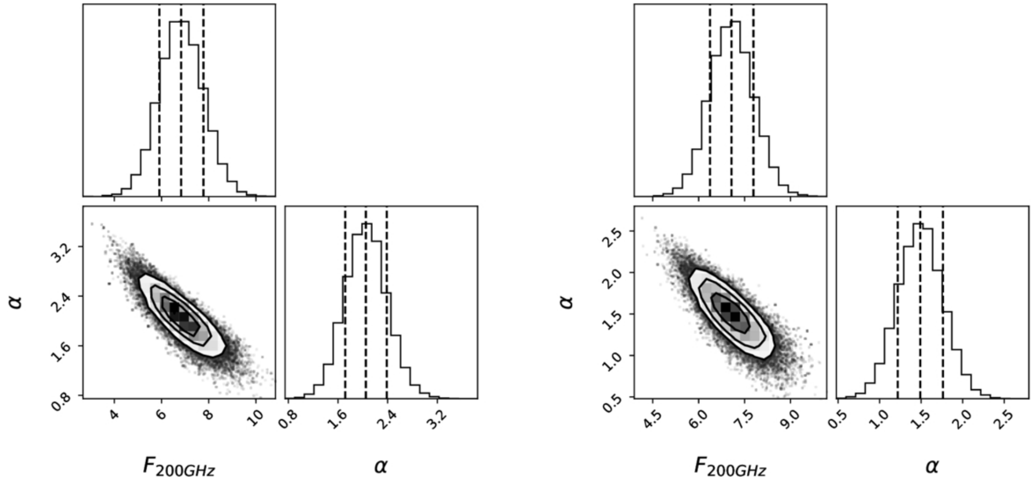
Figure 6. from Chia-Ying Chung et al 2026 Astron. J. 172 doi:10.3847/1538-3881/ae95f5 https://dx.doi.org/10.3847/1538-3881/ae95f5 © 2026. The Author(s). Published by the American Astronomical Society.
