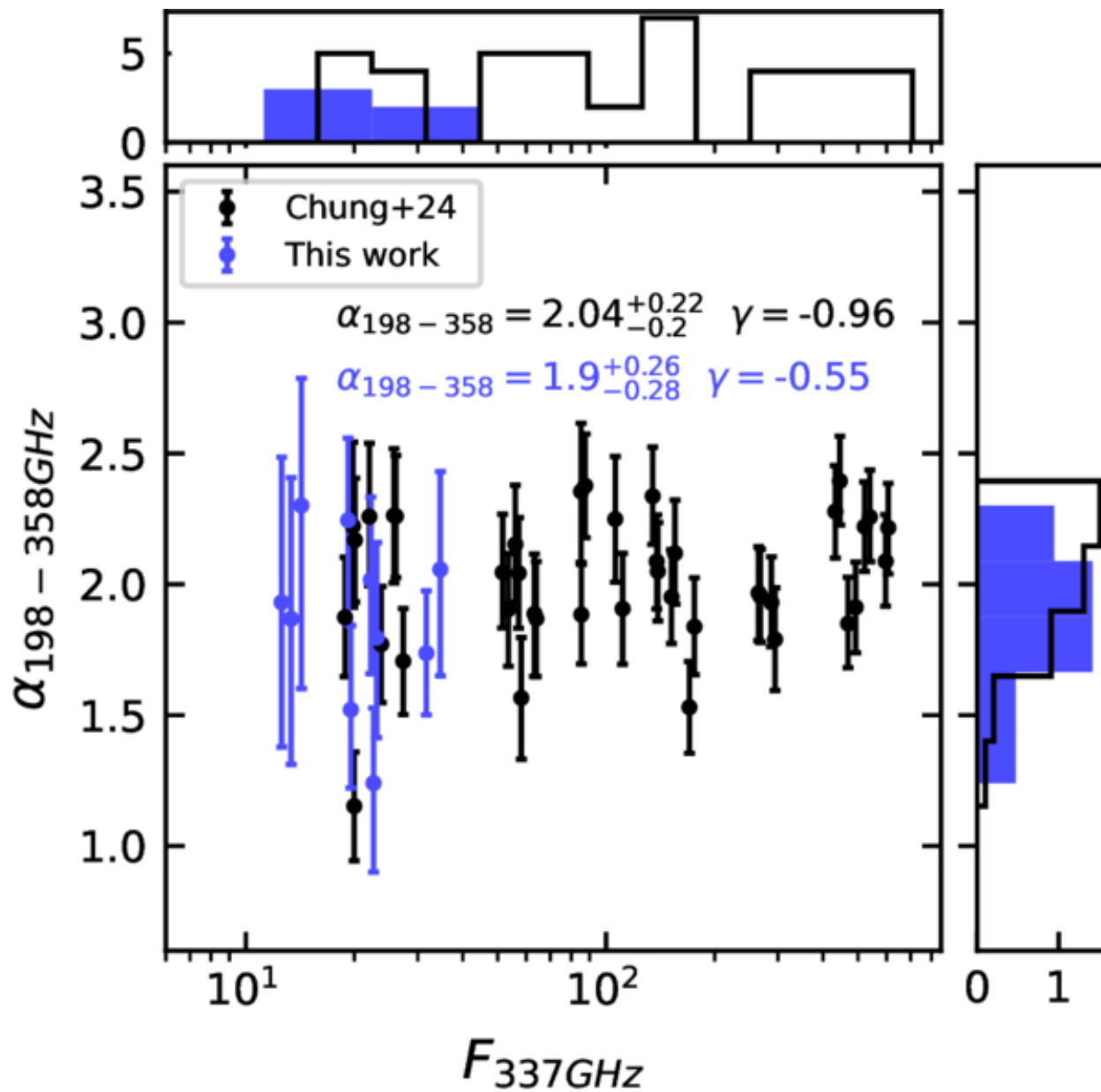
Figure 3. from Chia-Ying Chung et al 2026 Astron. J. 172 doi:10.3847/1538-3881/ae95f5 https://dx.doi.org/10.3847/1538-3881/ae95f5 © 2026. The Author(s). Published by the American Astronomical Society.
