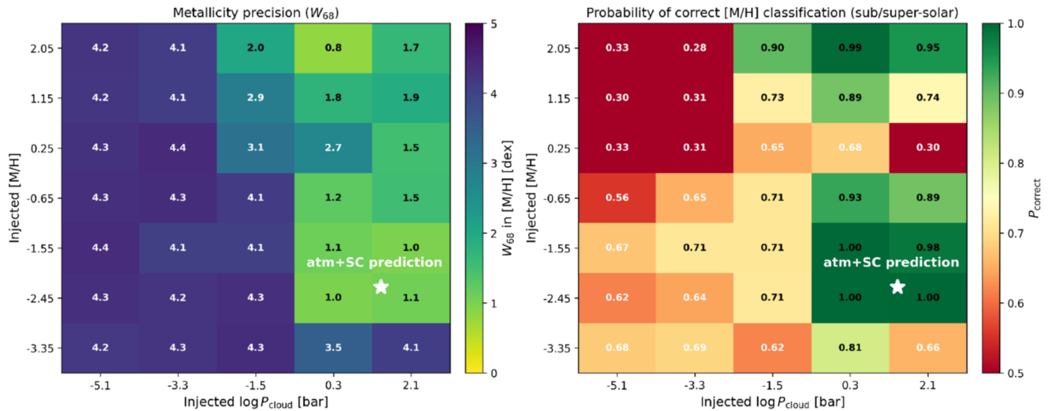
Figure 9. from Zoe Ko et al 2026 Astron. J. 172 doi:10.3847/1538-3881/ae9545 https://dx.doi.org/10.3847/1538-3881/ae9545 © 2026. The Author(s). Published by the American Astronomical Society.
