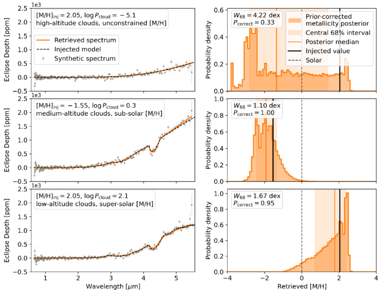
Figure 8. from Zoe Ko et al 2026 Astron. J. 172 doi:10.3847/1538-3881/ae9545 https://dx.doi.org/10.3847/1538-3881/ae9545 © 2026. The Author(s). Published by the American Astronomical Society.
