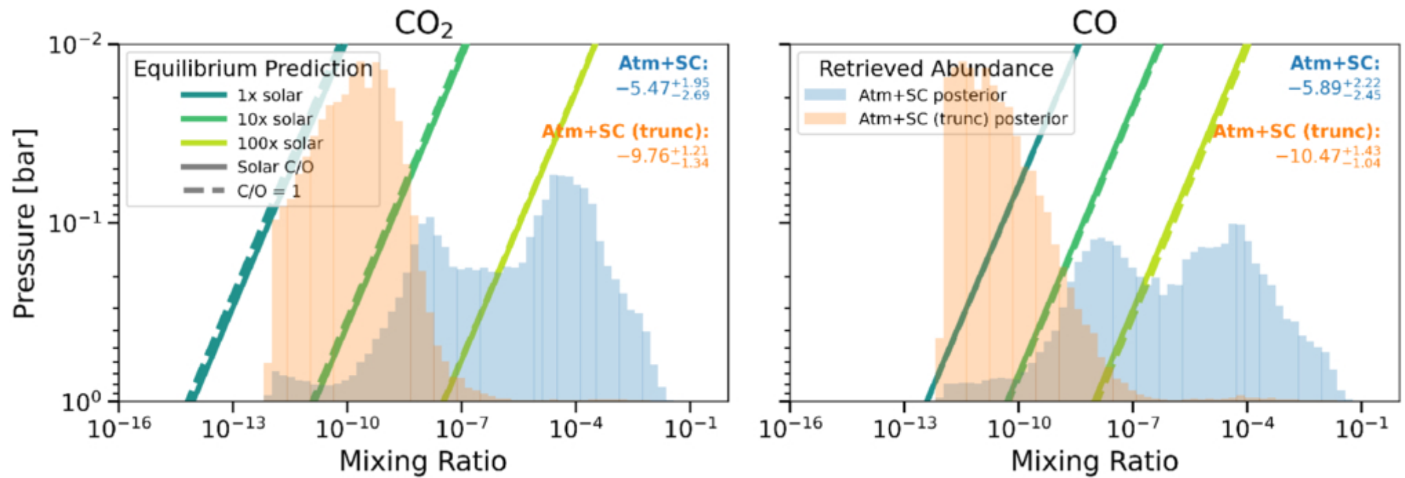
Figure 7. from Zoe Ko et al 2026 Astron. J. 172 doi:10.3847/1538-3881/ae9545 https://dx.doi.org/10.3847/1538-3881/ae9545 © 2026. The Author(s). Published by the American Astronomical Society.
