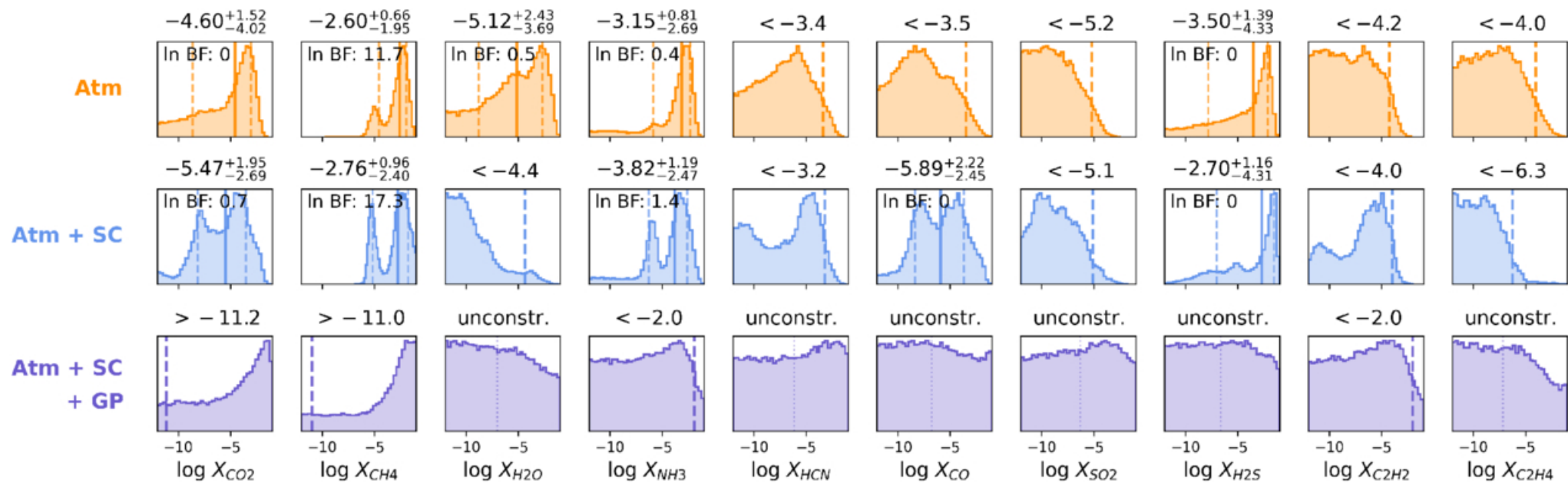
Figure 4. from Zoe Ko et al 2026 Astron. J. 172 doi:10.3847/1538-3881/ae9545 https://dx.doi.org/10.3847/1538-3881/ae9545 © 2026. The Author(s). Published by the American Astronomical Society.
