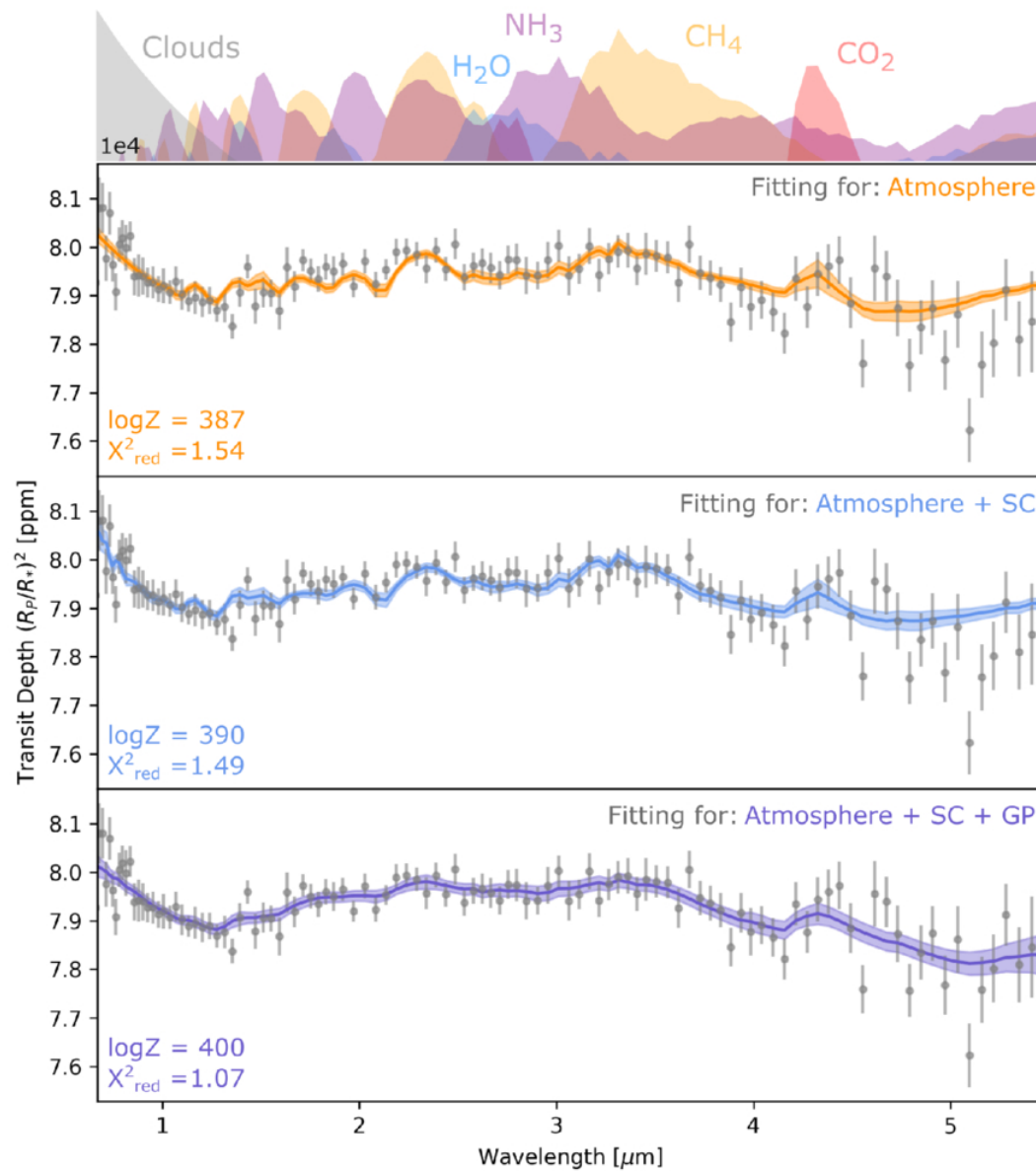
Figure 3. from Zoe Ko et al 2026 Astron. J. 172 doi:10.3847/1538-3881/ae9545 https://dx.doi.org/10.3847/1538-3881/ae9545 © 2026. The Author(s). Published by the American Astronomical Society.
