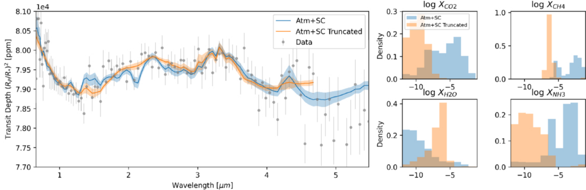
Figure 14. from Zoe Ko et al 2026 Astron. J. 172 doi:10.3847/1538-3881/ae9545 https://dx.doi.org/10.3847/1538-3881/ae9545 © 2026. The Author(s). Published by the American Astronomical Society.
