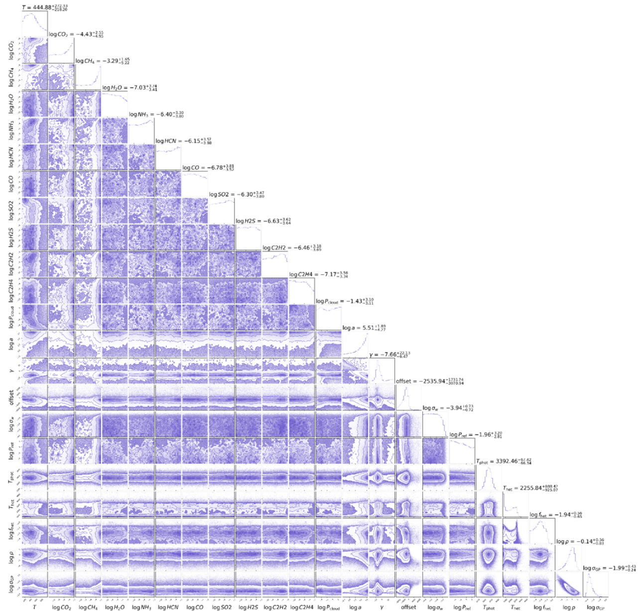
Figure 13. from Zoe Ko et al 2026 Astron. J. 172 doi:10.3847/1538-3881/ae9545 https://dx.doi.org/10.3847/1538-3881/ae9545 © 2026. The Author(s). Published by the American Astronomical Society.
