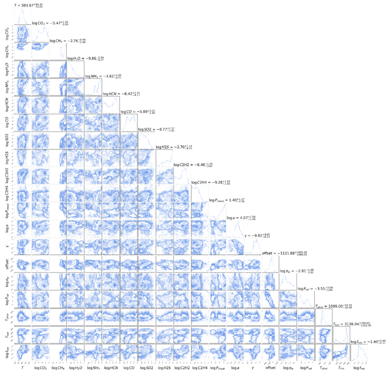
Figure 12. from Zoe Ko et al 2026 Astron. J. 172 doi:10.3847/1538-3881/ae9545 https://dx.doi.org/10.3847/1538-3881/ae9545 © 2026. The Author(s). Published by the American Astronomical Society.
