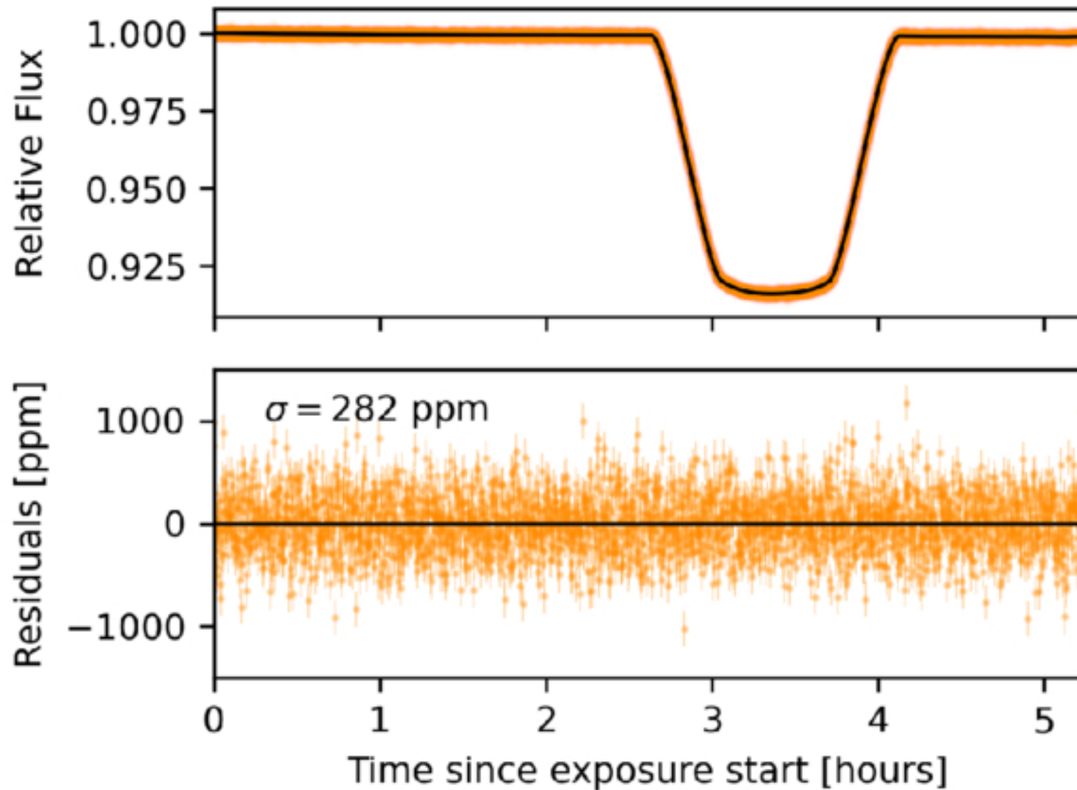
Figure 1. from Zoe Ko et al 2026 Astron. J. 172 doi:10.3847/1538-3881/ae9545 https://dx.doi.org/10.3847/1538-3881/ae9545 © 2026. The Author(s). Published by the American Astronomical Society.
