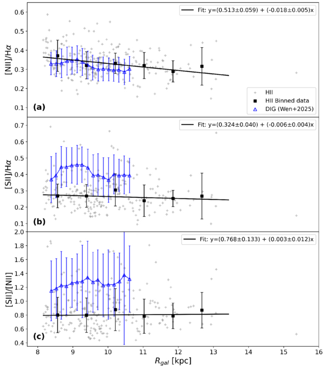
Figure 9. from Yunning Zhao et al 2026 Astron. J. 172 doi:10.3847/1538-3881/ae930f https://dx.doi.org/10.3847/1538-3881/ae930f © 2026. The Author(s). Published by the American Astronomical Society.
