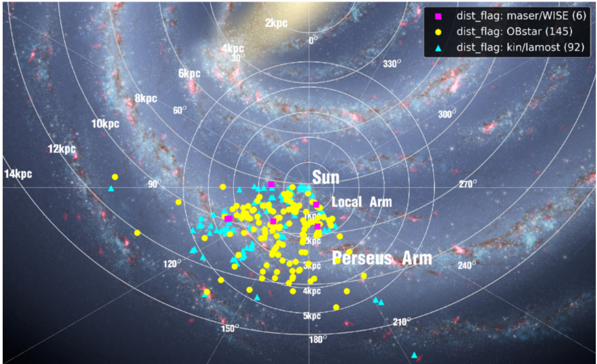
Figure 8. from Yunning Zhao et al 2026 Astron. J. 172 doi:10.3847/1538-3881/ae930f https://dx.doi.org/10.3847/1538-3881/ae930f © 2026. The Author(s). Published by the American Astronomical Society.
