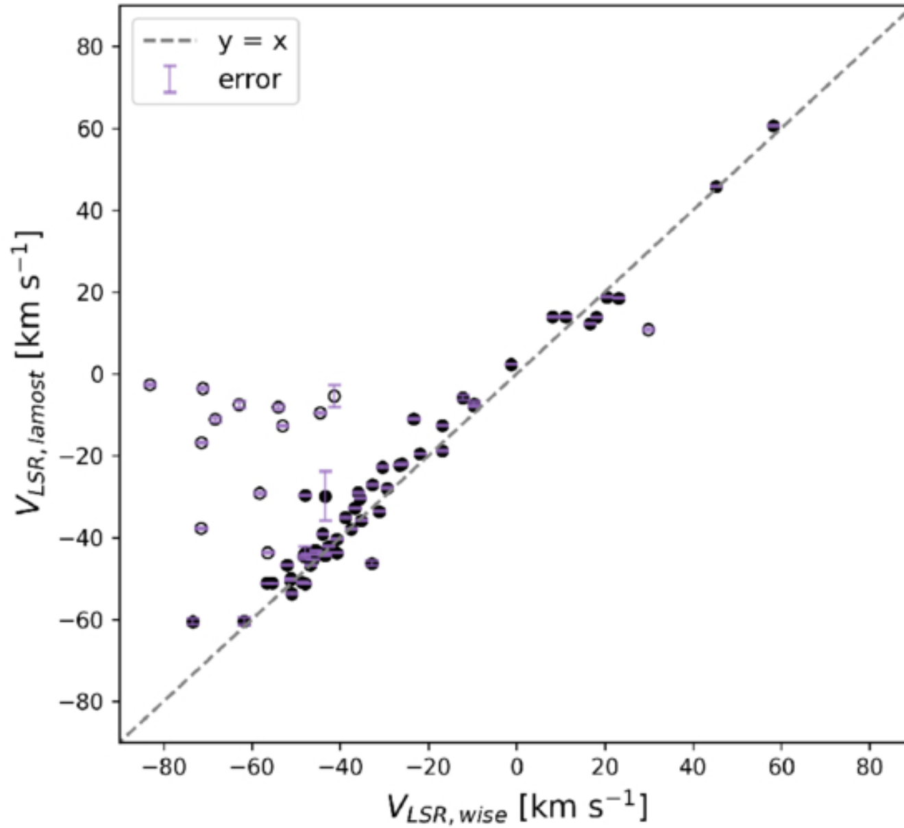
Figure 7. from Yunning Zhao et al 2026 Astron. J. 172 doi:10.3847/1538-3881/ae930f https://dx.doi.org/10.3847/1538-3881/ae930f © 2026. The Author(s). Published by the American Astronomical Society.
