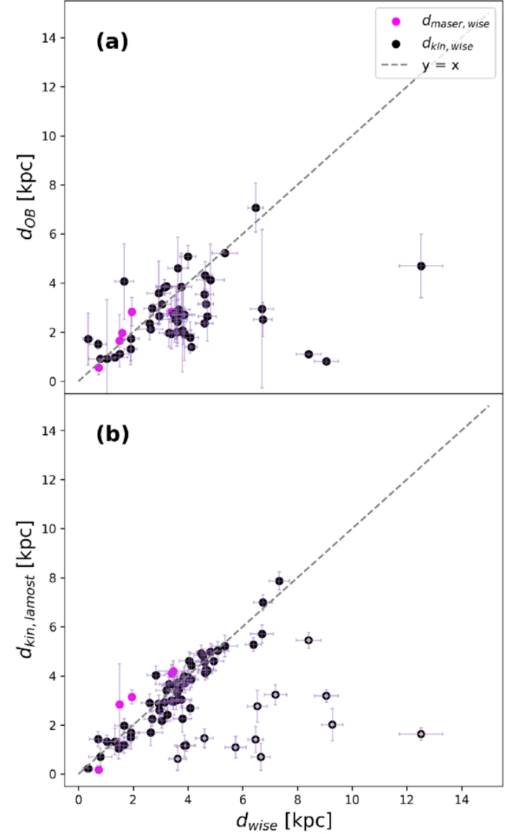
Figure 6. from Yunning Zhao et al 2026 Astron. J. 172 doi:10.3847/1538-3881/ae930f https://dx.doi.org/10.3847/1538-3881/ae930f © 2026. The Author(s). Published by the American Astronomical Society.
