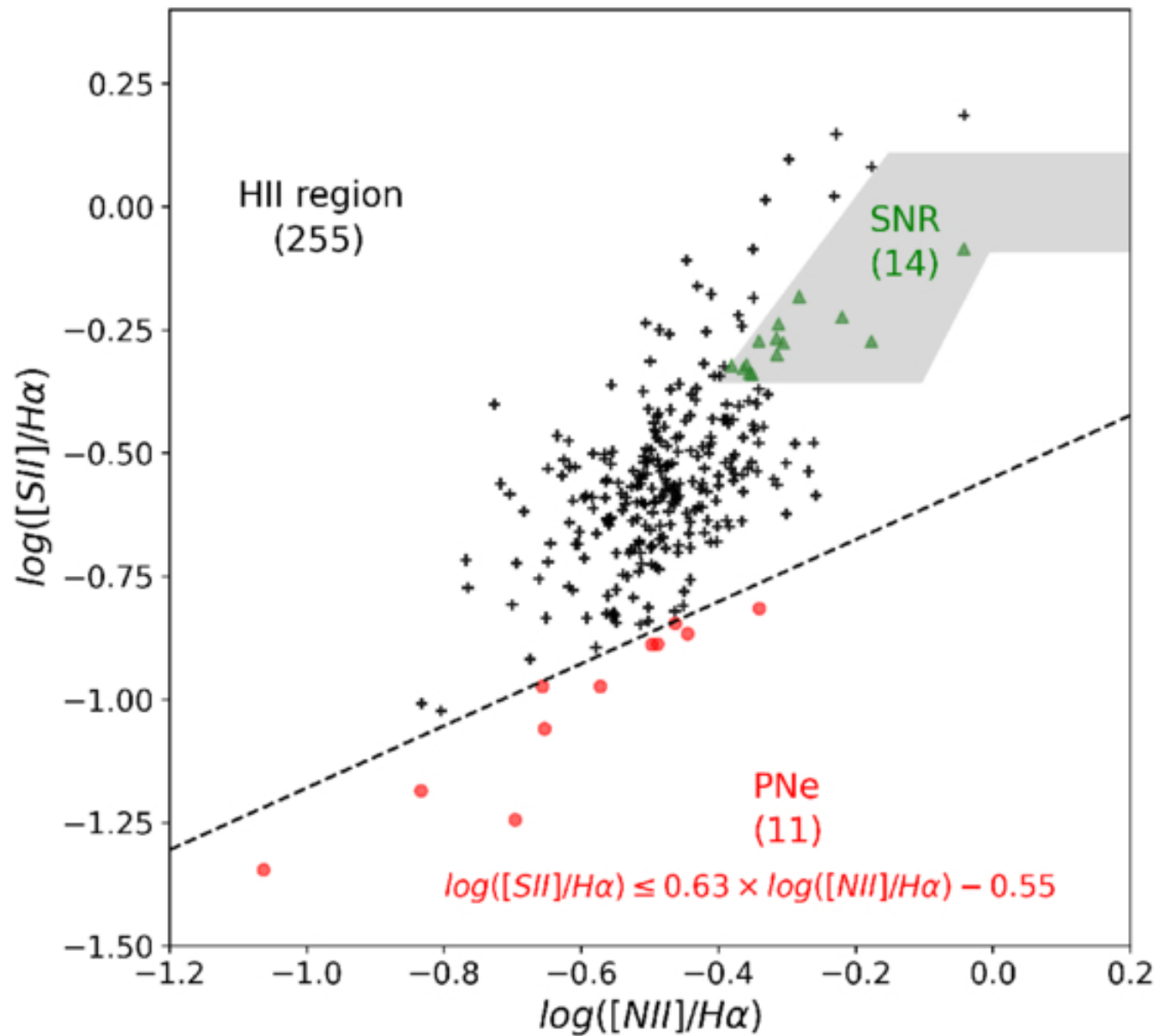
Figure 4. from Yunning Zhao et al 2026 Astron. J. 172 doi:10.3847/1538-3881/ae930f https://dx.doi.org/10.3847/1538-3881/ae930f © 2026. The Author(s). Published by the American Astronomical Society.
