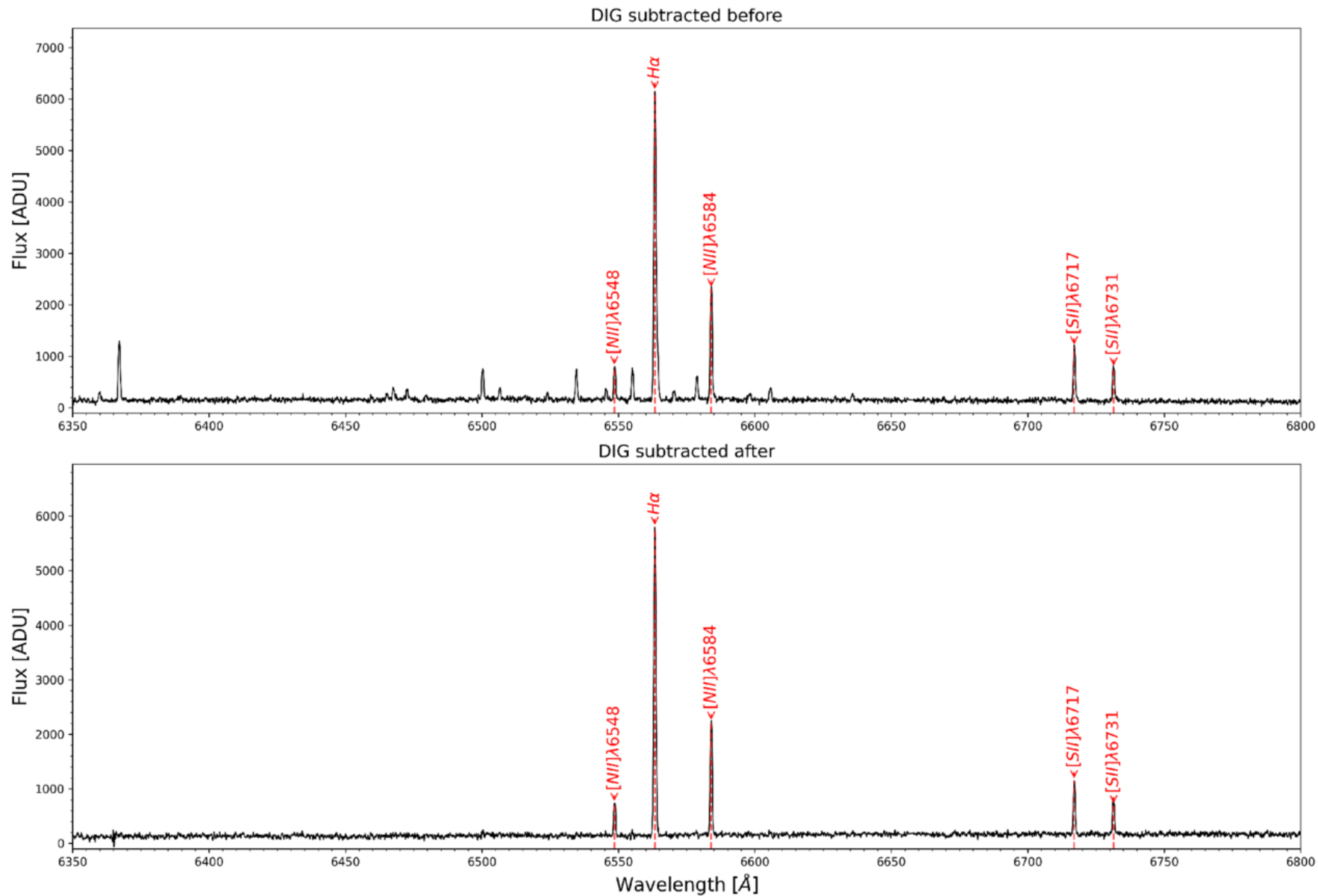
Figure 2. from Yunning Zhao et al 2026 Astron. J. 172 doi:10.3847/1538-3881/ae930f https://dx.doi.org/10.3847/1538-3881/ae930f © 2026. The Author(s). Published by the American Astronomical Society.
