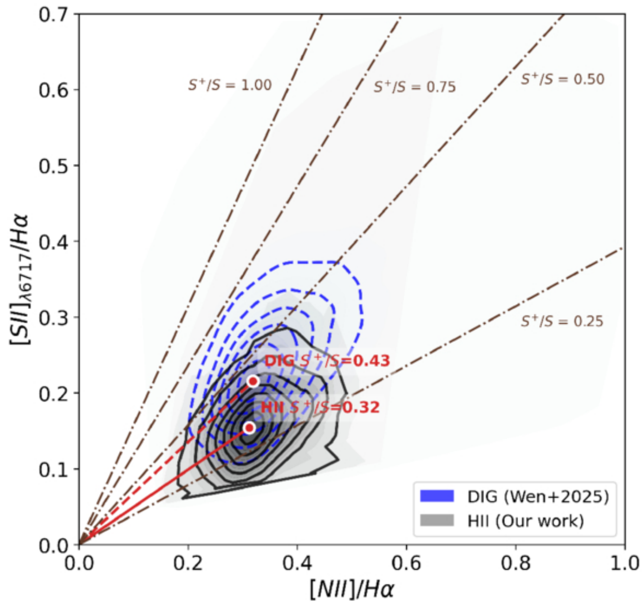
Figure 13. from Yunning Zhao et al 2026 Astron. J. 172 doi:10.3847/1538-3881/ae930f https://dx.doi.org/10.3847/1538-3881/ae930f © 2026. The Author(s). Published by the American Astronomical Society.
