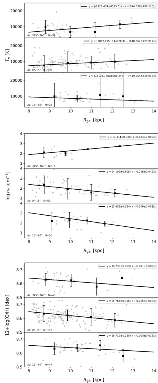
Figure 12. from Yunning Zhao et al 2026 Astron. J. 172 doi:10.3847/1538-3881/ae930f https://dx.doi.org/10.3847/1538-3881/ae930f © 2026. The Author(s). Published by the American Astronomical Society.
