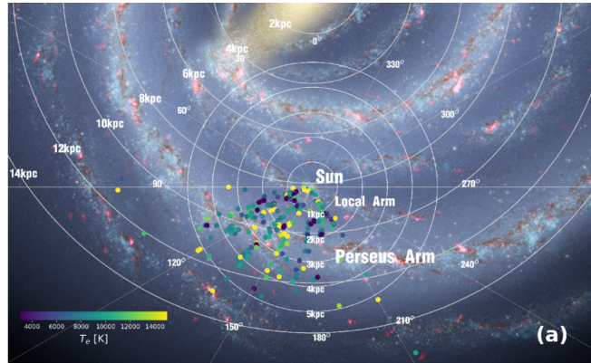
Figure 11. from Yunning Zhao et al 2026 Astron. J. 172 doi:10.3847/1538-3881/ae930f https://dx.doi.org/10.3847/1538-3881/ae930f © 2026. The Author(s). Published by the American Astronomical Society.
