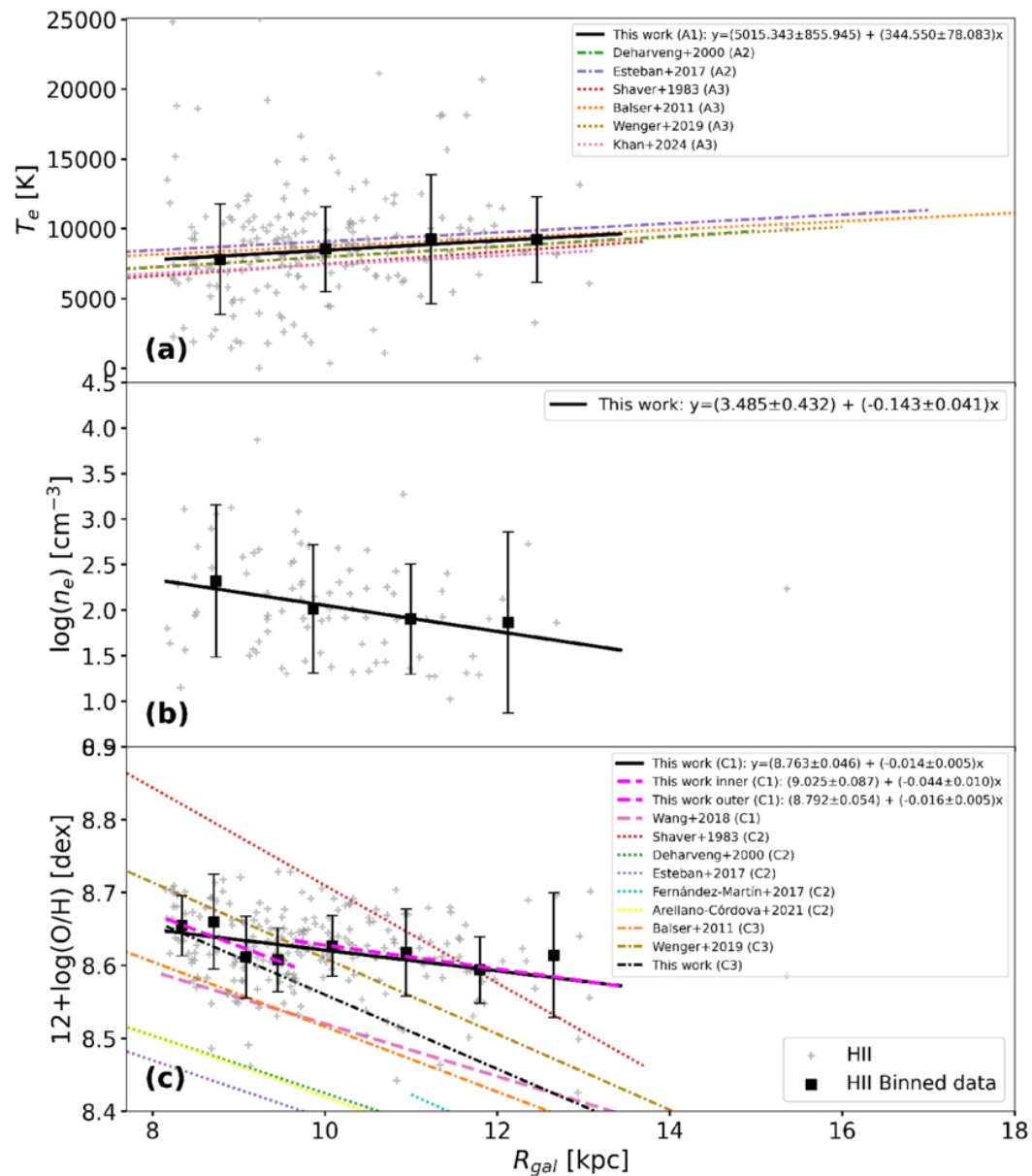
Figure 10. from Yunning Zhao et al 2026 Astron. J. 172 doi:10.3847/1538-3881/ae930f https://dx.doi.org/10.3847/1538-3881/ae930f © 2026. The Author(s). Published by the American Astronomical Society.
