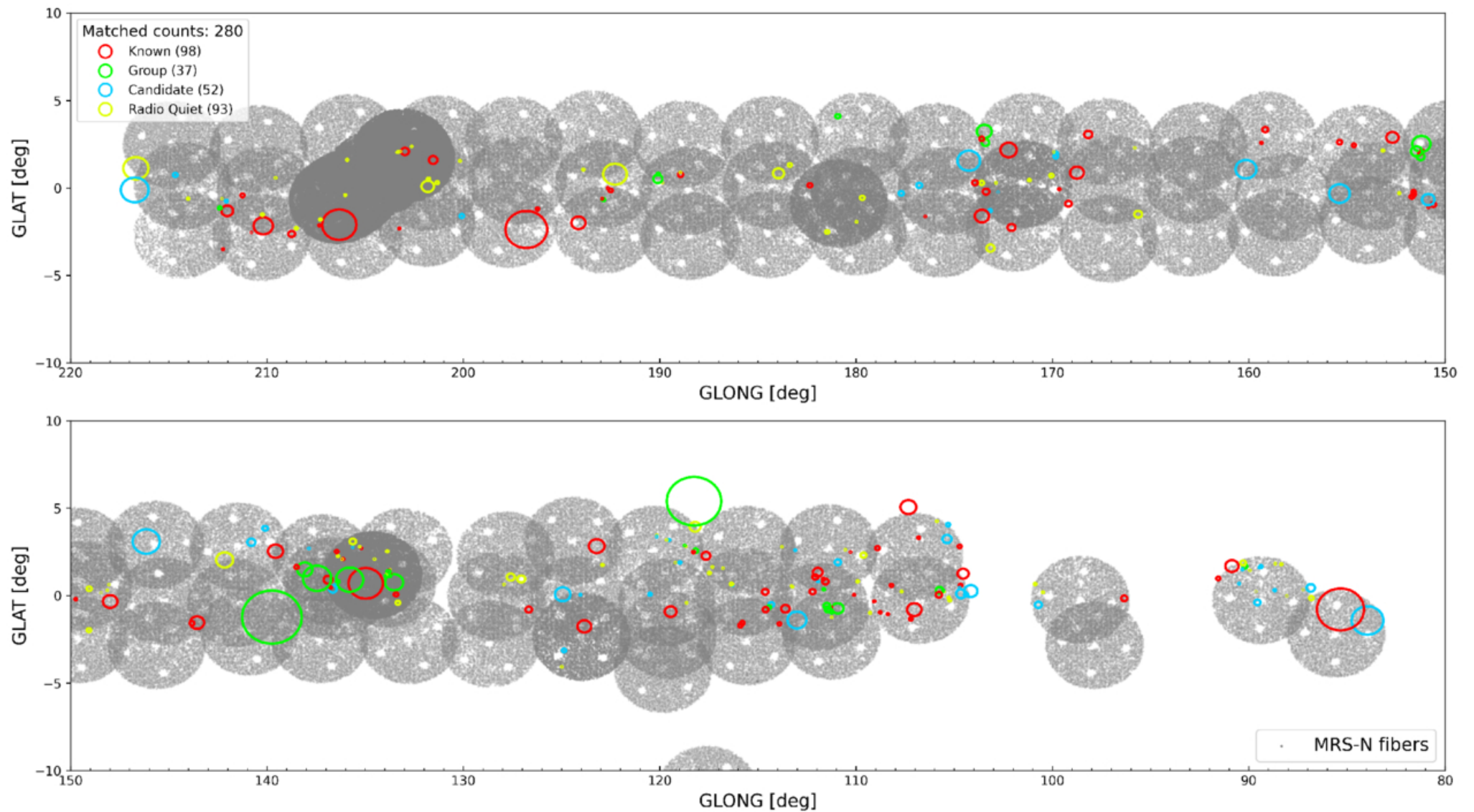
Figure 1. from Yunning Zhao et al 2026 Astron. J. 172 doi:10.3847/1538-3881/ae930f https://dx.doi.org/10.3847/1538-3881/ae930f © 2026. The Author(s). Published by the American Astronomical Society.
