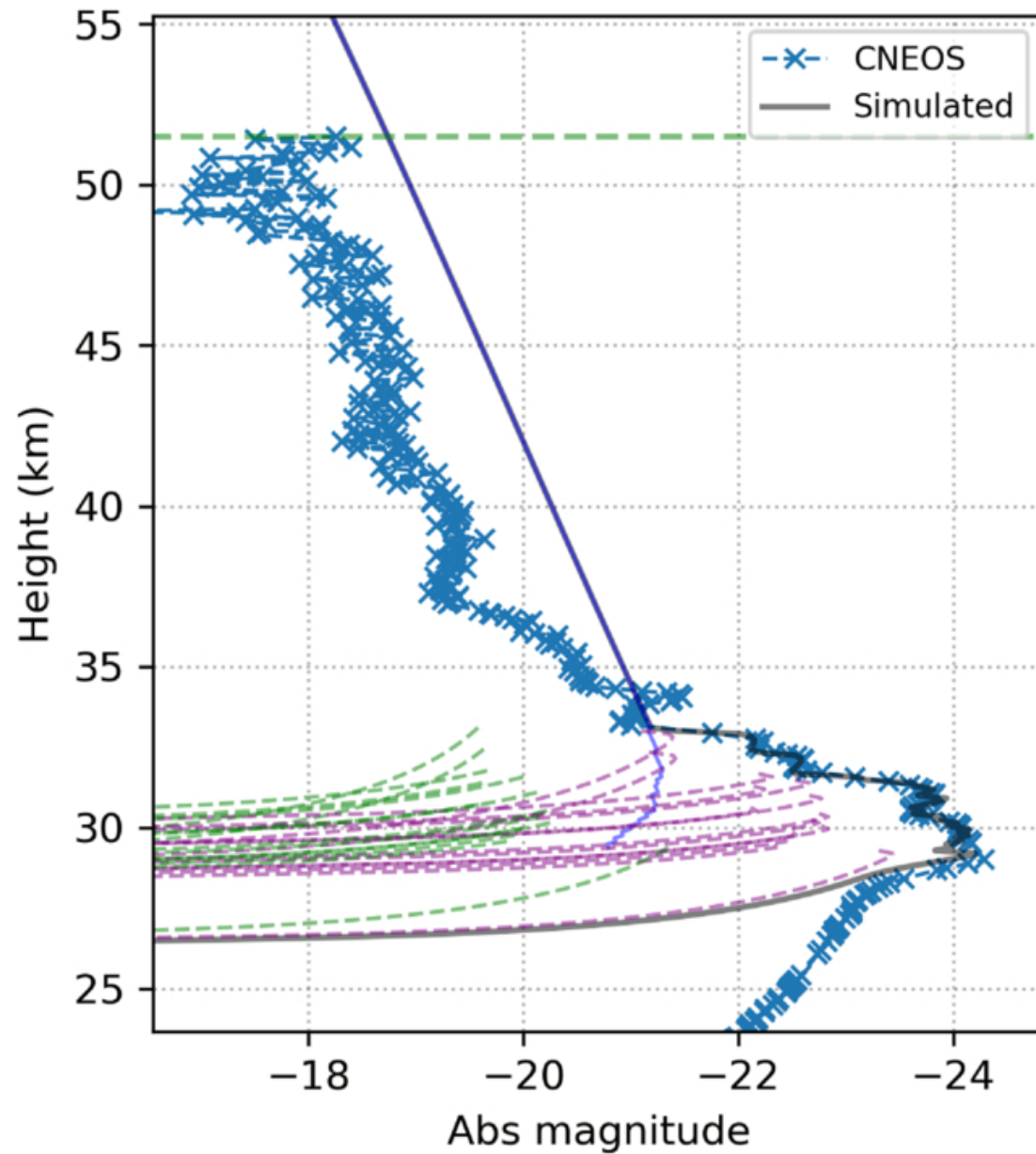
Figure 7. from Elizabeth A. Silber et al 2026 Astron. J. 172 doi:10.3847/1538-3881/ae9285 https://dx.doi.org/10.3847/1538-3881/ae9285 © 2026. The Author(s). Published by the American Astronomical Society.
