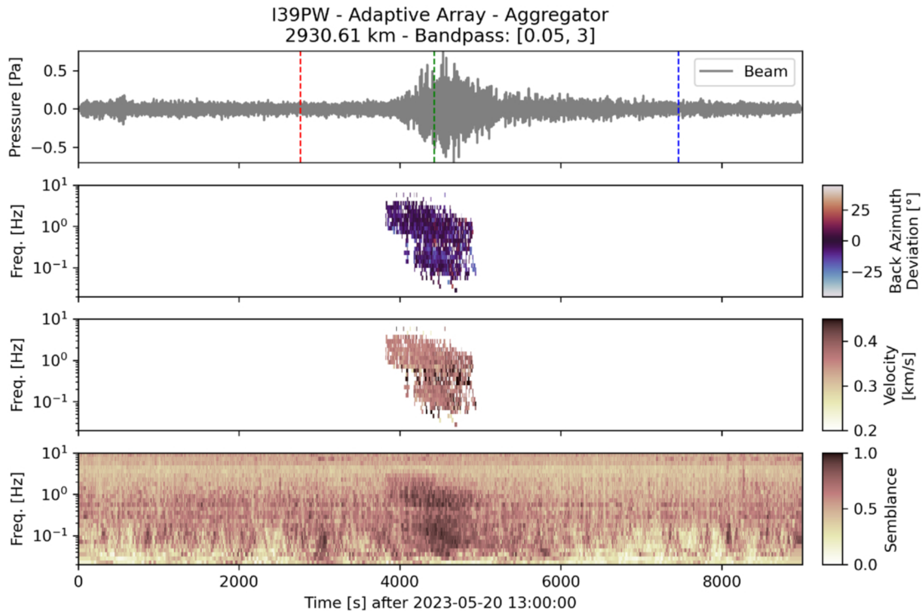
Figure 5. from Elizabeth A. Silber et al 2026 Astron. J. 172 doi:10.3847/1538-3881/ae9285 https://dx.doi.org/10.3847/1538-3881/ae9285 © 2026. The Author(s). Published by the American Astronomical Society.
