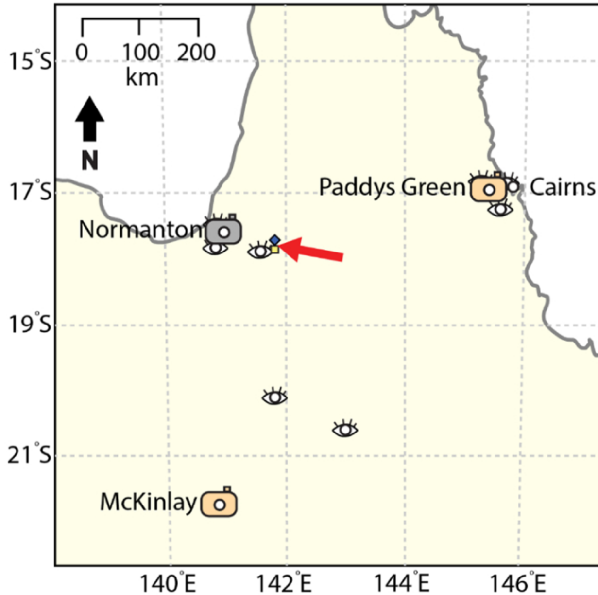
Figure 2. from Elizabeth A. Silber et al 2026 Astron. J. 172 doi:10.3847/1538-3881/ae9285 https://dx.doi.org/10.3847/1538-3881/ae9285 © 2026. The Author(s). Published by the American Astronomical Society.
