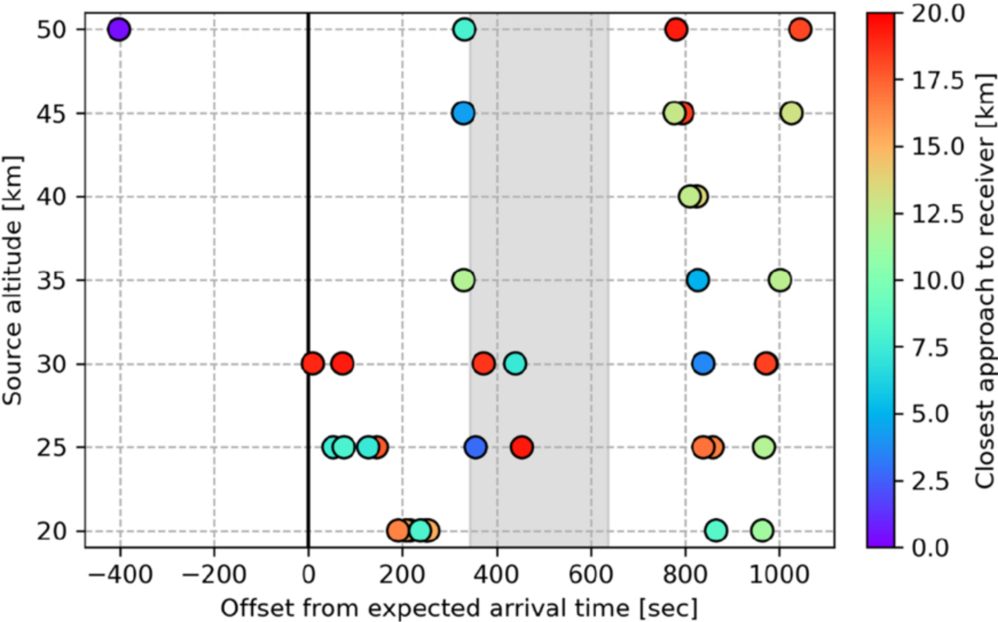
Figure B3. from Elizabeth A. Silber et al 2026 Astron. J. 172 doi:10.3847/1538-3881/ae9285 https://dx.doi.org/10.3847/1538-3881/ae9285 © 2026. The Author(s). Published by the American Astronomical Society.
