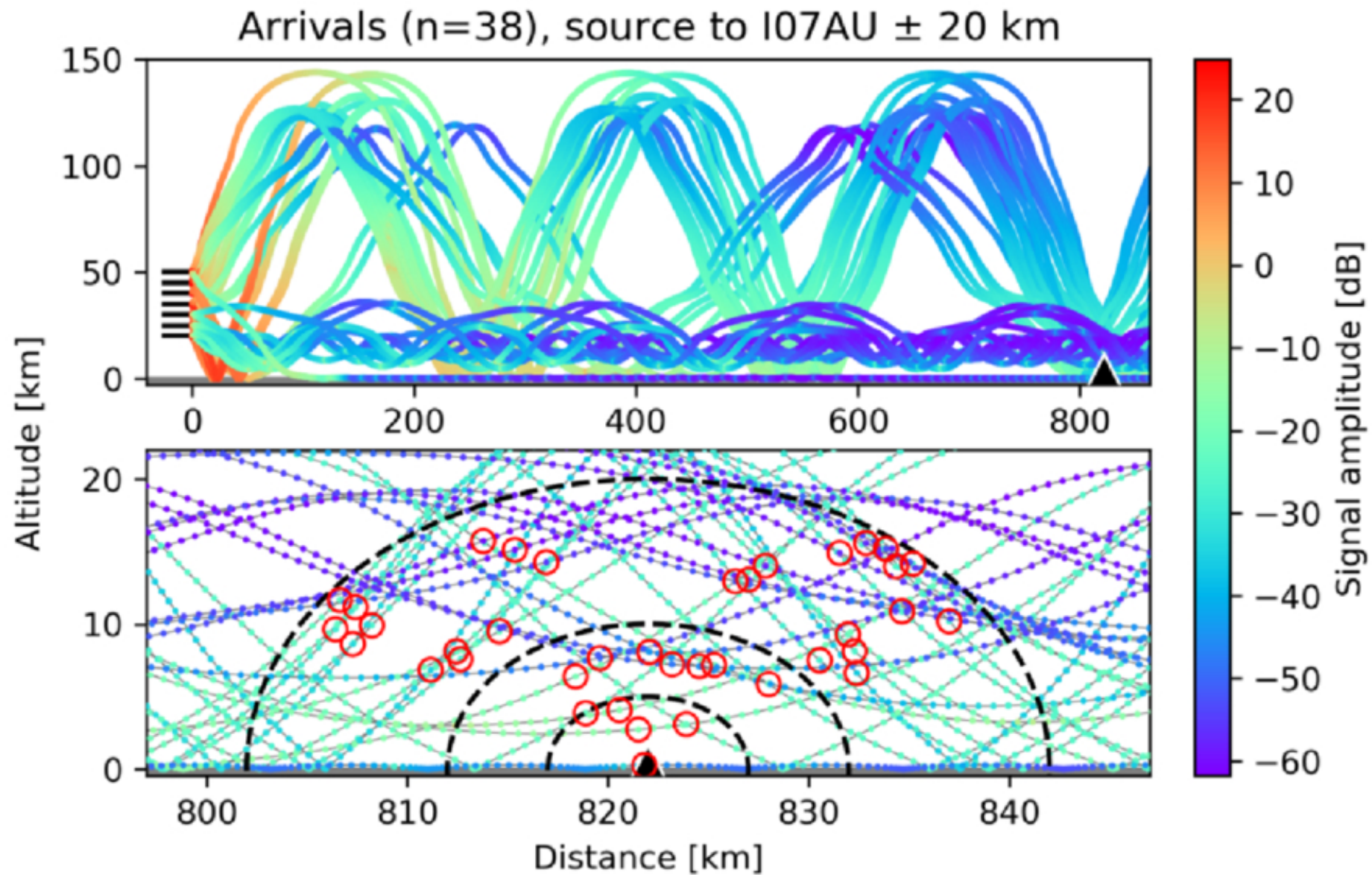
Figure B1. from Elizabeth A. Silber et al 2026 Astron. J. 172 doi:10.3847/1538-3881/ae9285 https://dx.doi.org/10.3847/1538-3881/ae9285 © 2026. The Author(s). Published by the American Astronomical Society.
