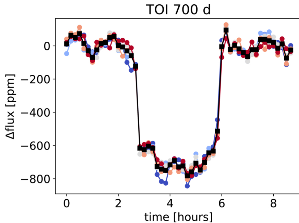
Figure 6. from Emily K. Pass et al 2026 Astron. J. 172 doi:10.3847/1538-3881/ae9283 https://dx.doi.org/10.3847/1538-3881/ae9283 © 2026. The Author(s). Published by the American Astronomical Society.
