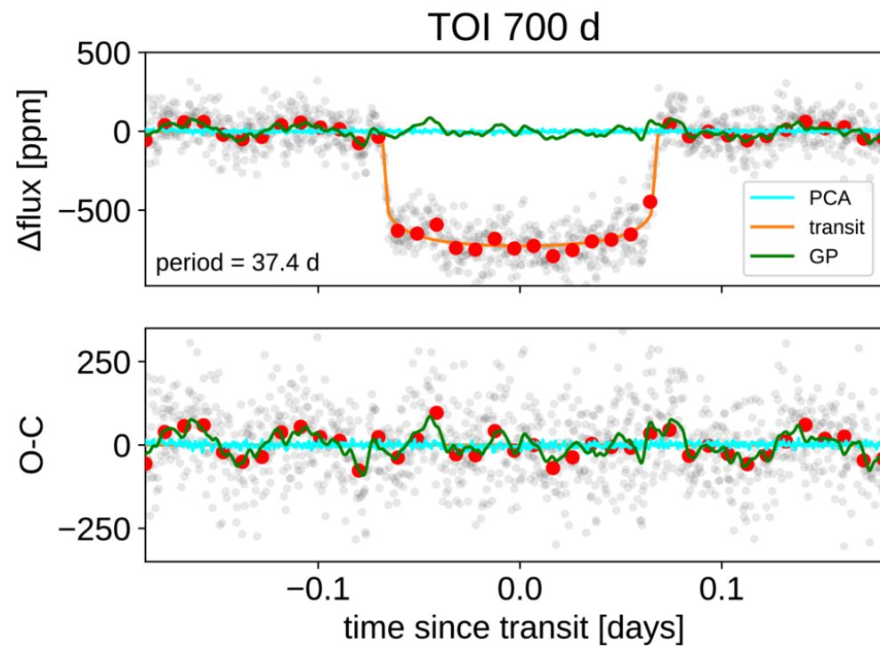
Figure 4. from Emily K. Pass et al 2026 Astron. J. 172 doi:10.3847/1538-3881/ae9283 https://dx.doi.org/10.3847/1538-3881/ae9283 © 2026. The Author(s). Published by the American Astronomical Society.
