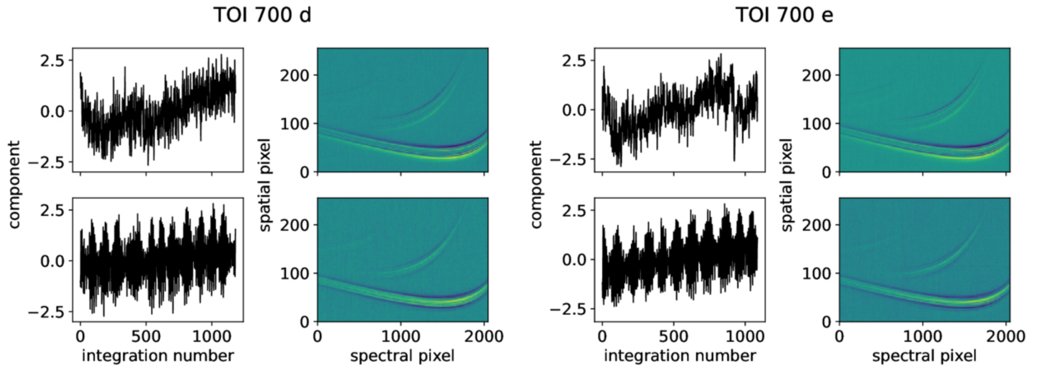
Figure 3. from Emily K. Pass et al 2026 Astron. J. 172 doi:10.3847/1538-3881/ae9283 https://dx.doi.org/10.3847/1538-3881/ae9283 © 2026. The Author(s). Published by the American Astronomical Society.
