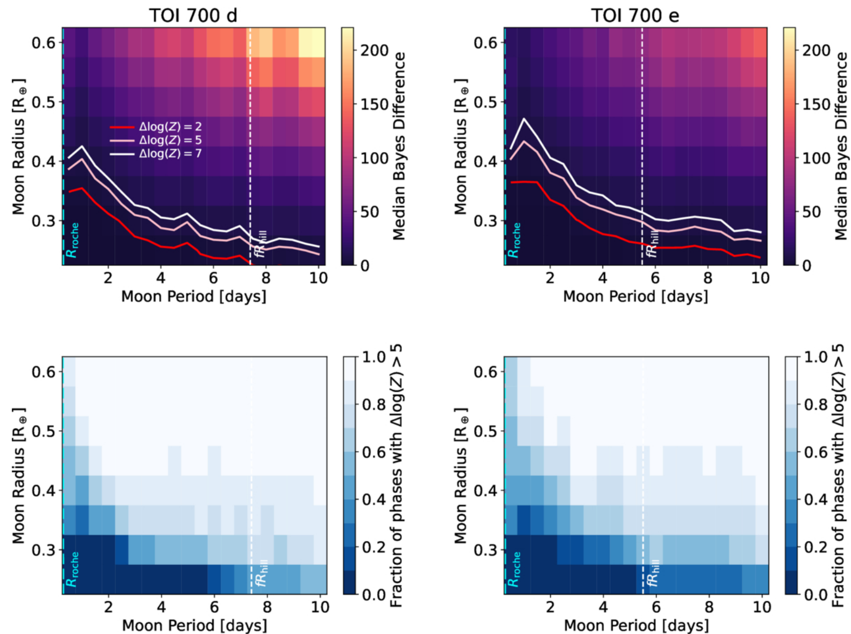
Figure 11. from Emily K. Pass et al 2026 Astron. J. 172 doi:10.3847/1538-3881/ae9283 https://dx.doi.org/10.3847/1538-3881/ae9283 © 2026. The Author(s). Published by the American Astronomical Society.
