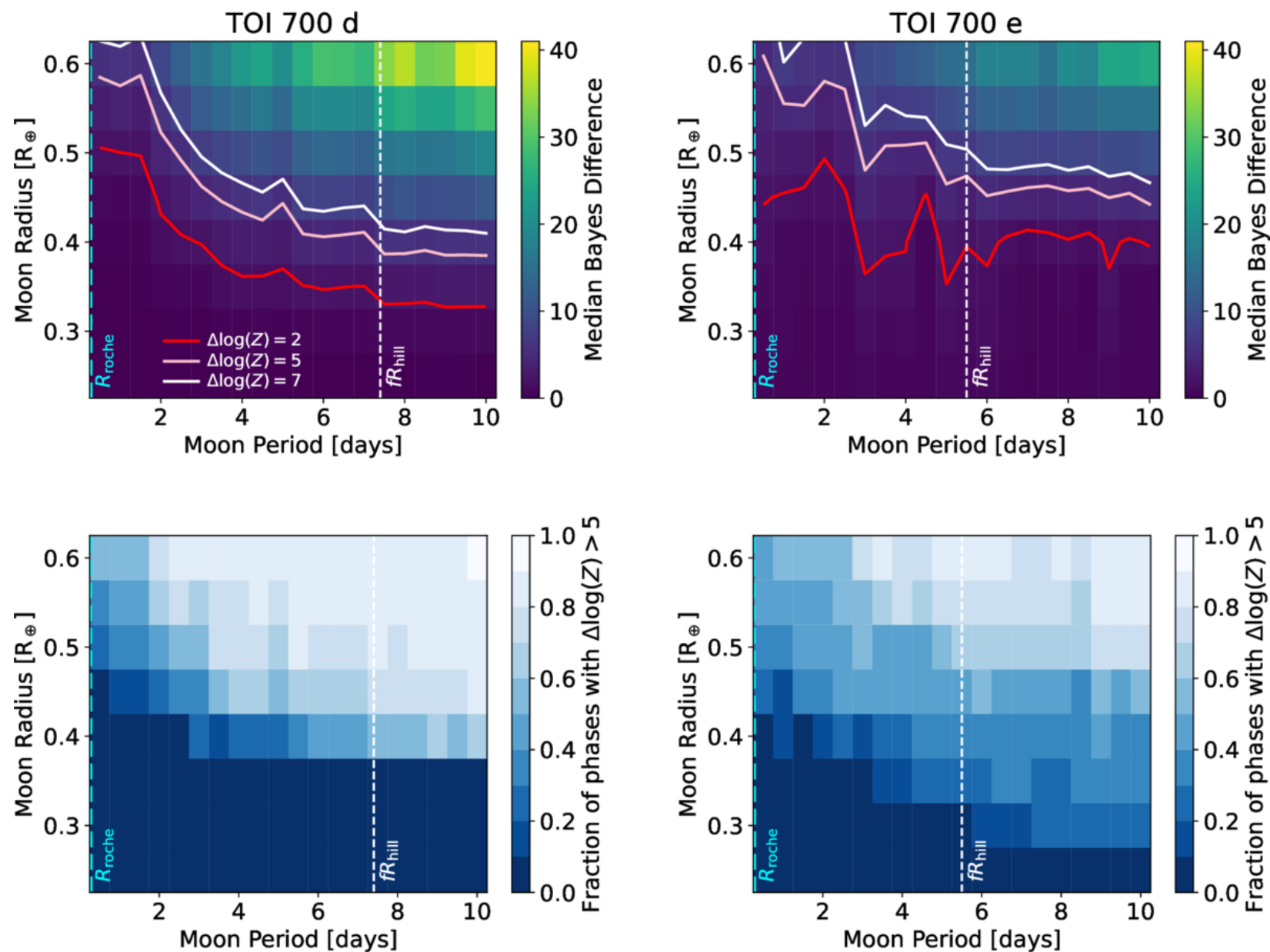
Figure 10. from Emily K. Pass et al 2026 Astron. J. 172 doi:10.3847/1538-3881/ae9283 https://dx.doi.org/10.3847/1538-3881/ae9283 © 2026. The Author(s). Published by the American Astronomical Society.
