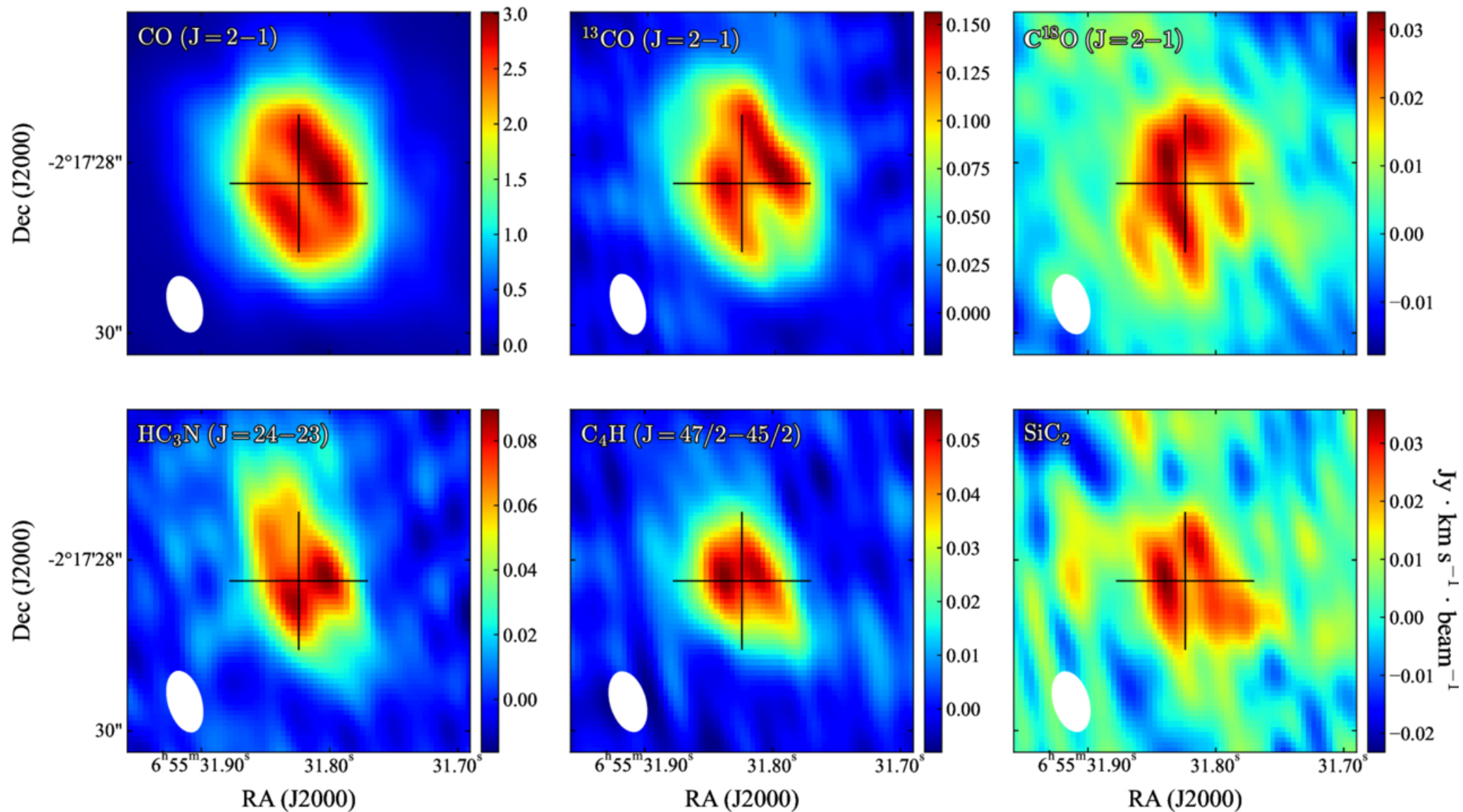
Figure 9. from Hao-Min Sun et al 2026 Astron. J. 172 doi:10.3847/1538-3881/ae91d0 https://dx.doi.org/10.3847/1538-3881/ae91d0 © 2026. The Author(s). Published by the American Astronomical Society.
