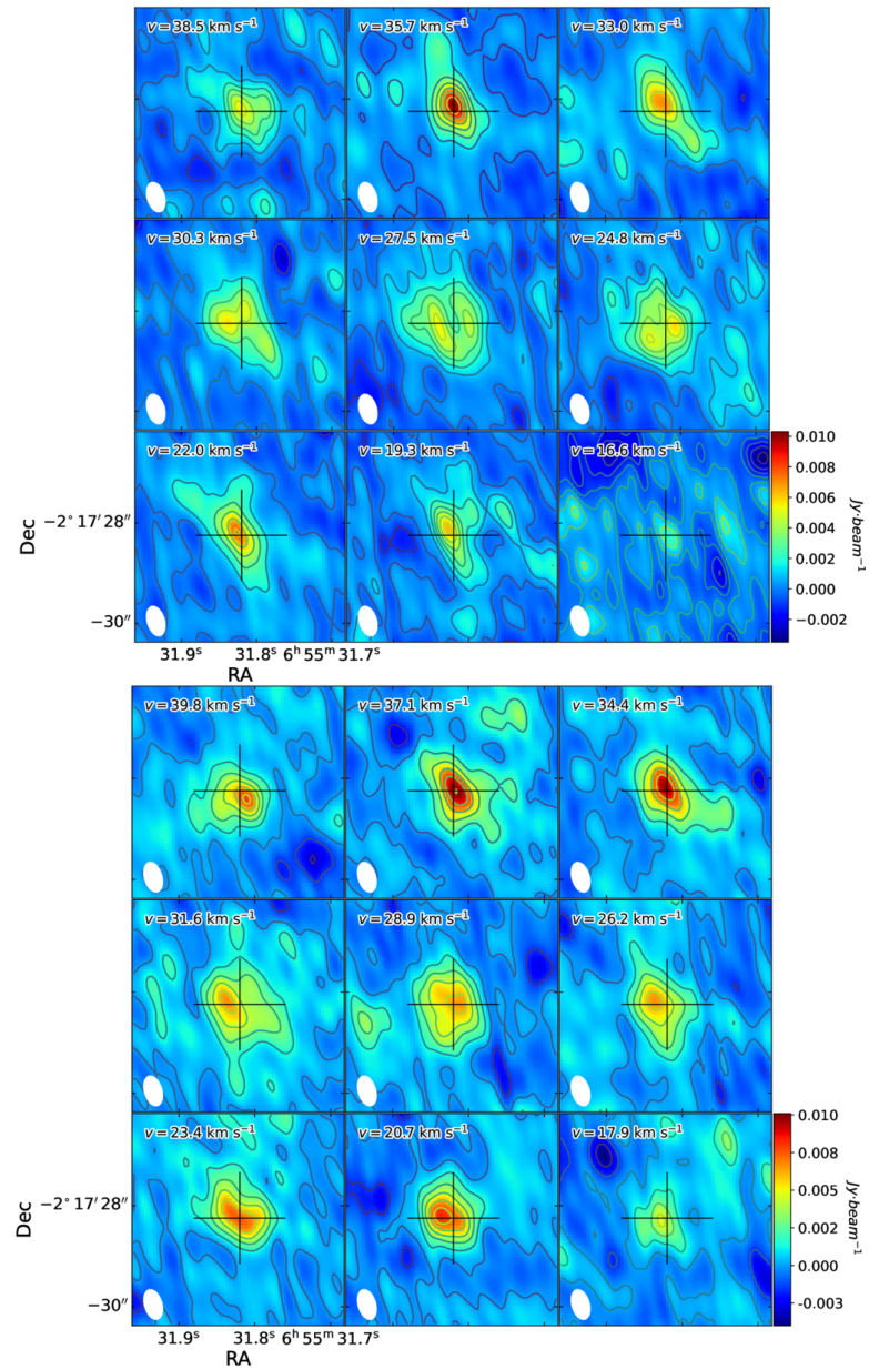
Figure 6. from Hao-Min Sun et al 2026 Astron. J. 172 doi:10.3847/1538-3881/ae91d0 https://dx.doi.org/10.3847/1538-3881/ae91d0 © 2026. The Author(s). Published by the American Astronomical Society.
