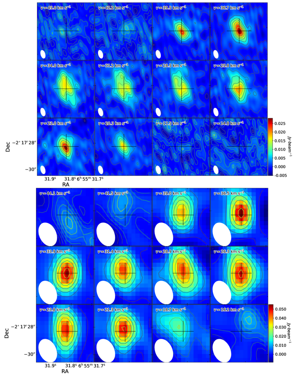
Figure 4. from Hao-Min Sun et al 2026 Astron. J. 172 doi:10.3847/1538-3881/ae91d0 https://dx.doi.org/10.3847/1538-3881/ae91d0 © 2026. The Author(s). Published by the American Astronomical Society.
