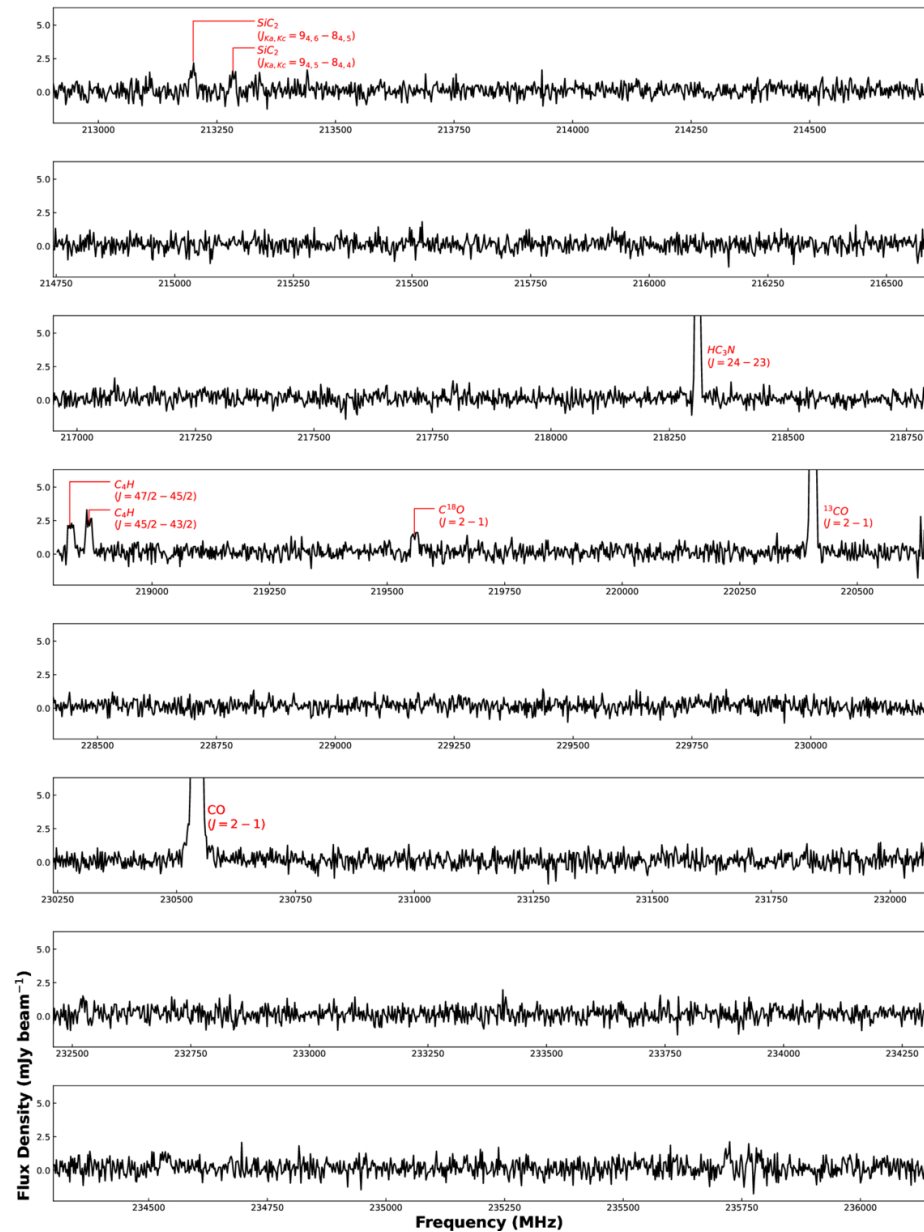
Figure 2. from Hao-Min Sun et al 2026 Astron. J. 172 doi:10.3847/1538-3881/ae91d0 https://dx.doi.org/10.3847/1538-3881/ae91d0 © 2026. The Author(s). Published by the American Astronomical Society.
