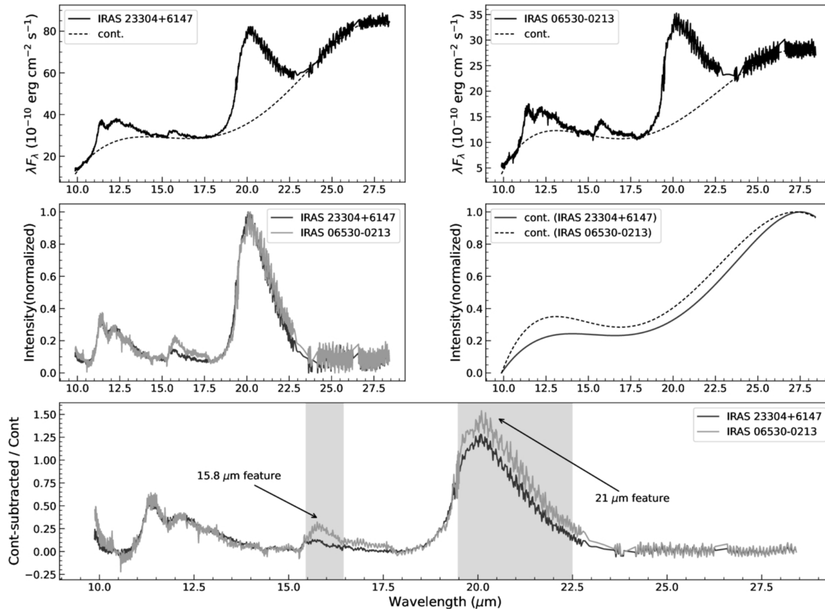
Figure 11. from Hao-Min Sun et al 2026 Astron. J. 172 doi:10.3847/1538-3881/ae91d0 https://dx.doi.org/10.3847/1538-3881/ae91d0 © 2026. The Author(s). Published by the American Astronomical Society.
