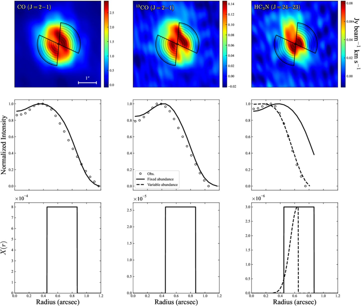
Figure 10. from Hao-Min Sun et al 2026 Astron. J. 172 doi:10.3847/1538-3881/ae91d0 https://dx.doi.org/10.3847/1538-3881/ae91d0 © 2026. The Author(s). Published by the American Astronomical Society.
