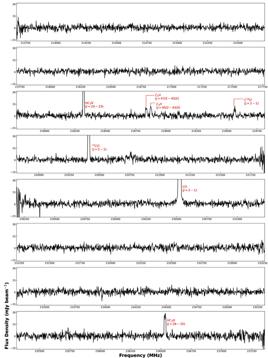
Figure 1. from Hao-Min Sun et al 2026 Astron. J. 172 doi:10.3847/1538-3881/ae91d0 https://dx.doi.org/10.3847/1538-3881/ae91d0 © 2026. The Author(s). Published by the American Astronomical Society.
