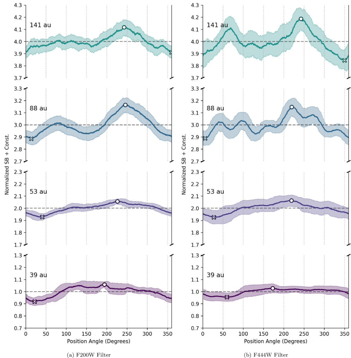
Figure 9. from Yu-Chia Lin et al 2026 Astron. J. 172 doi:10.3847/1538-3881/ae90a6 https://dx.doi.org/10.3847/1538-3881/ae90a6 © 2026. The Author(s). Published by the American Astronomical Society.
