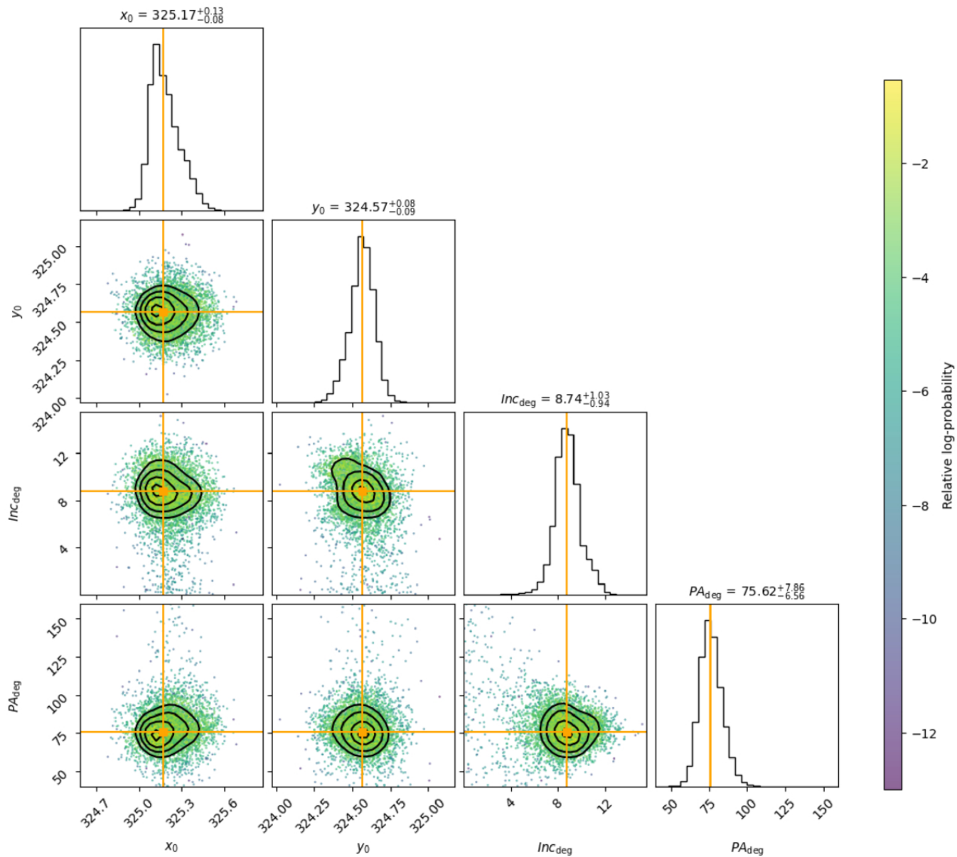
Figure 5. from Yu-Chia Lin et al 2026 Astron. J. 172 doi:10.3847/1538-3881/ae90a6 https://dx.doi.org/10.3847/1538-3881/ae90a6 © 2026. The Author(s). Published by the American Astronomical Society.
