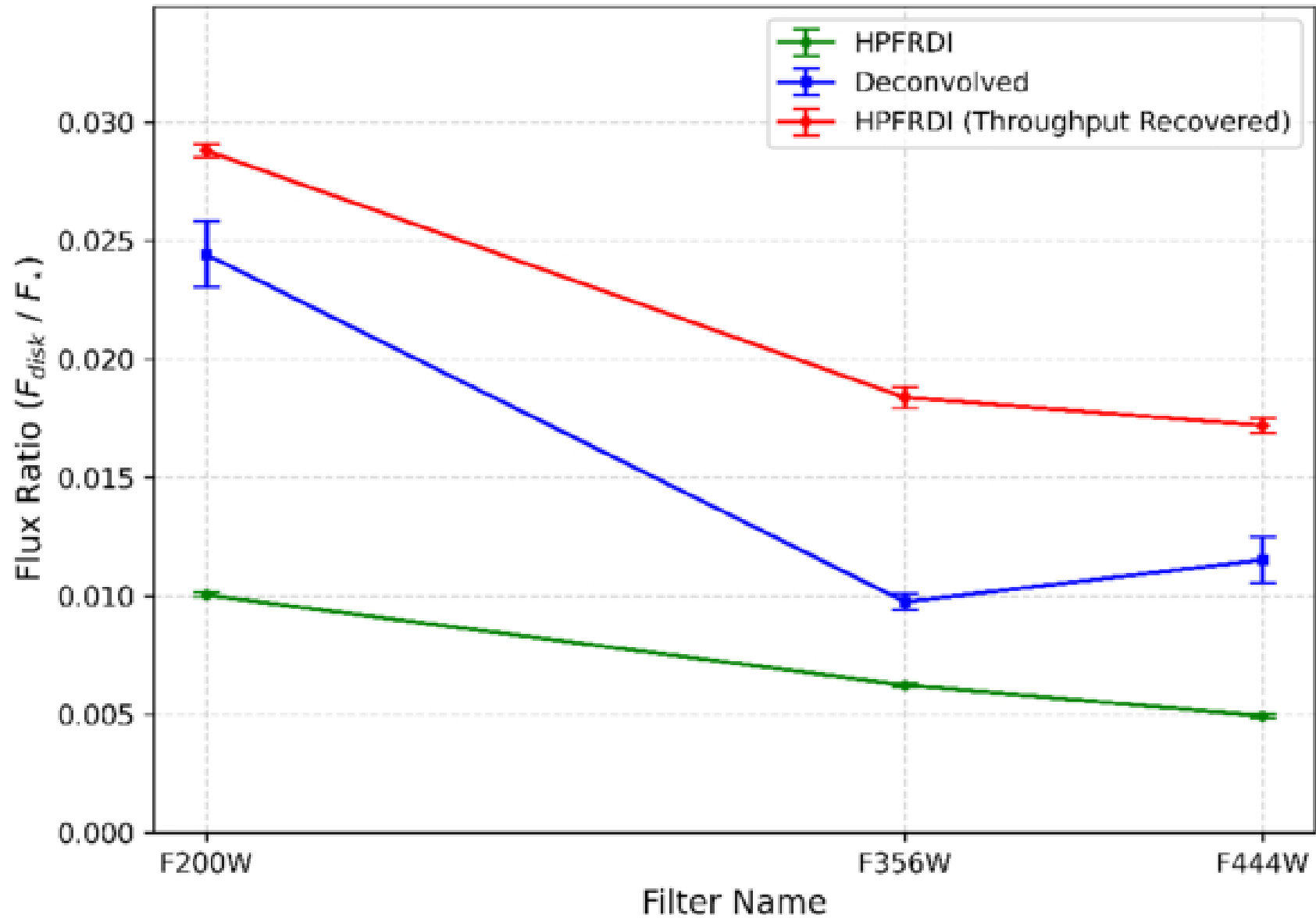
Figure 2. from Yu-Chia Lin et al 2026 Astron. J. 172 doi:10.3847/1538-3881/ae90a6 https://dx.doi.org/10.3847/1538-3881/ae90a6 © 2026. The Author(s). Published by the American Astronomical Society.
