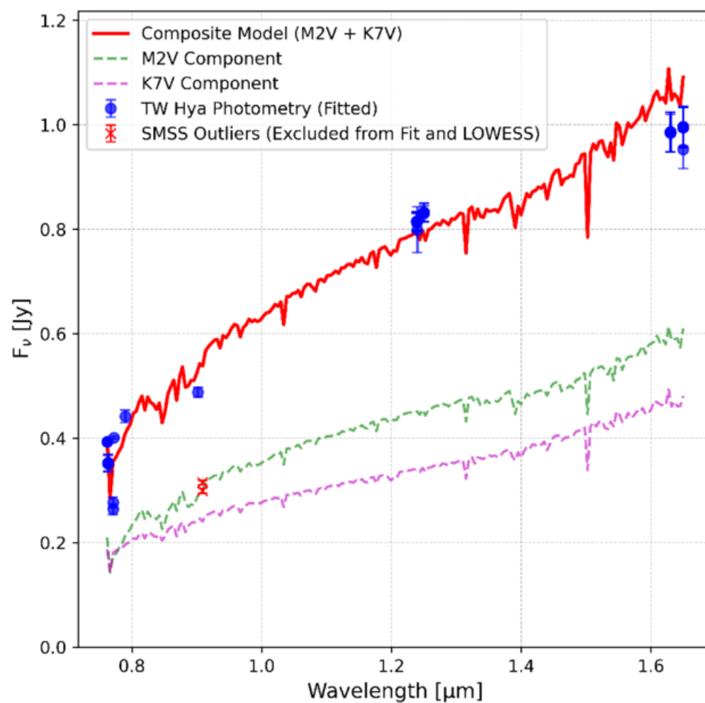
Figure 14. from Yu-Chia Lin et al 2026 Astron. J. 172 doi:10.3847/1538-3881/ae90a6 https://dx.doi.org/10.3847/1538-3881/ae90a6 © 2026. The Author(s). Published by the American Astronomical Society.
