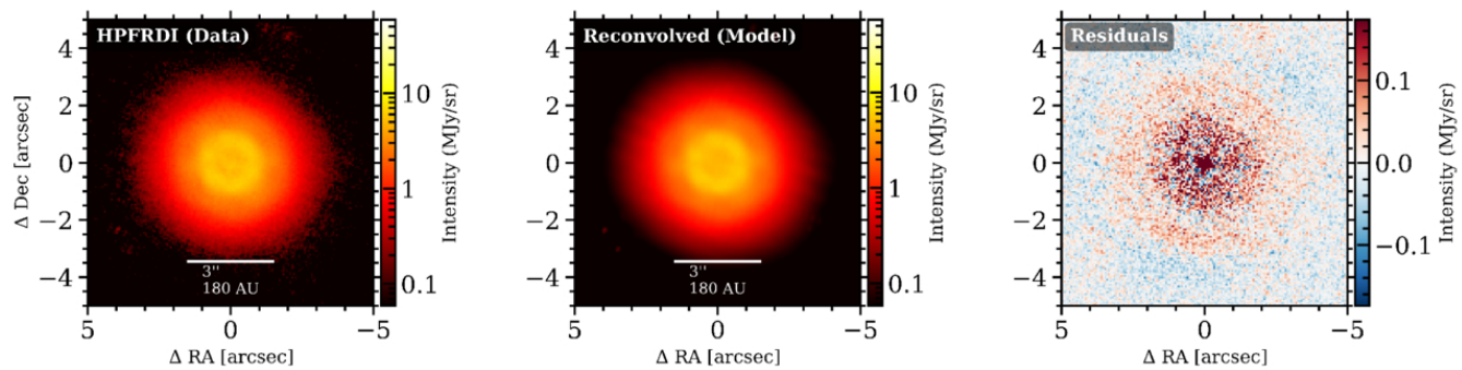
(c) F444W
