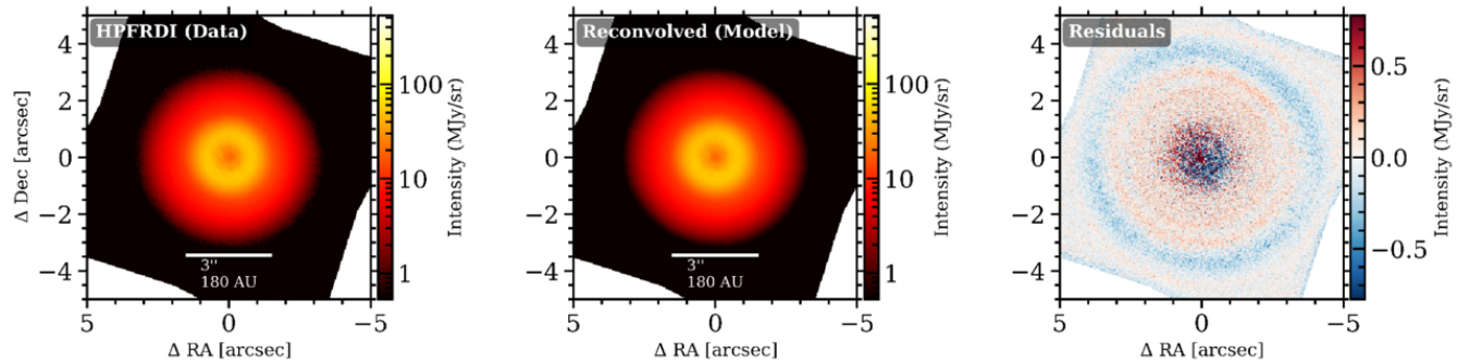
(a) F200W
