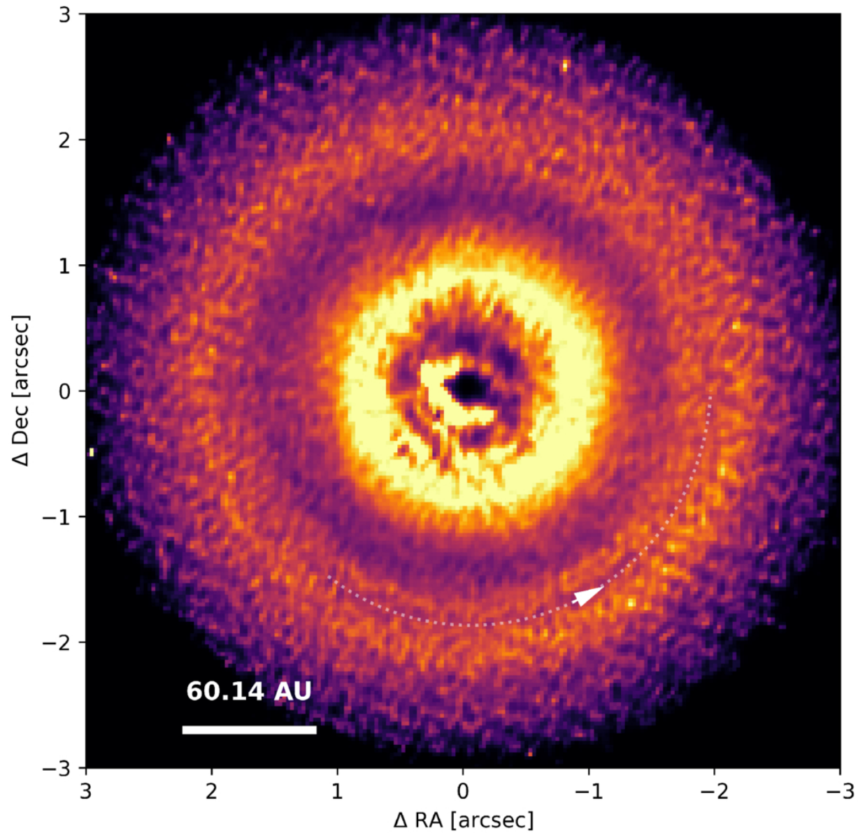
Figure 10. from Yu-Chia Lin et al 2026 Astron. J. 172 doi:10.3847/1538-3881/ae90a6 https://dx.doi.org/10.3847/1538-3881/ae90a6 © 2026. The Author(s). Published by the American Astronomical Society.
