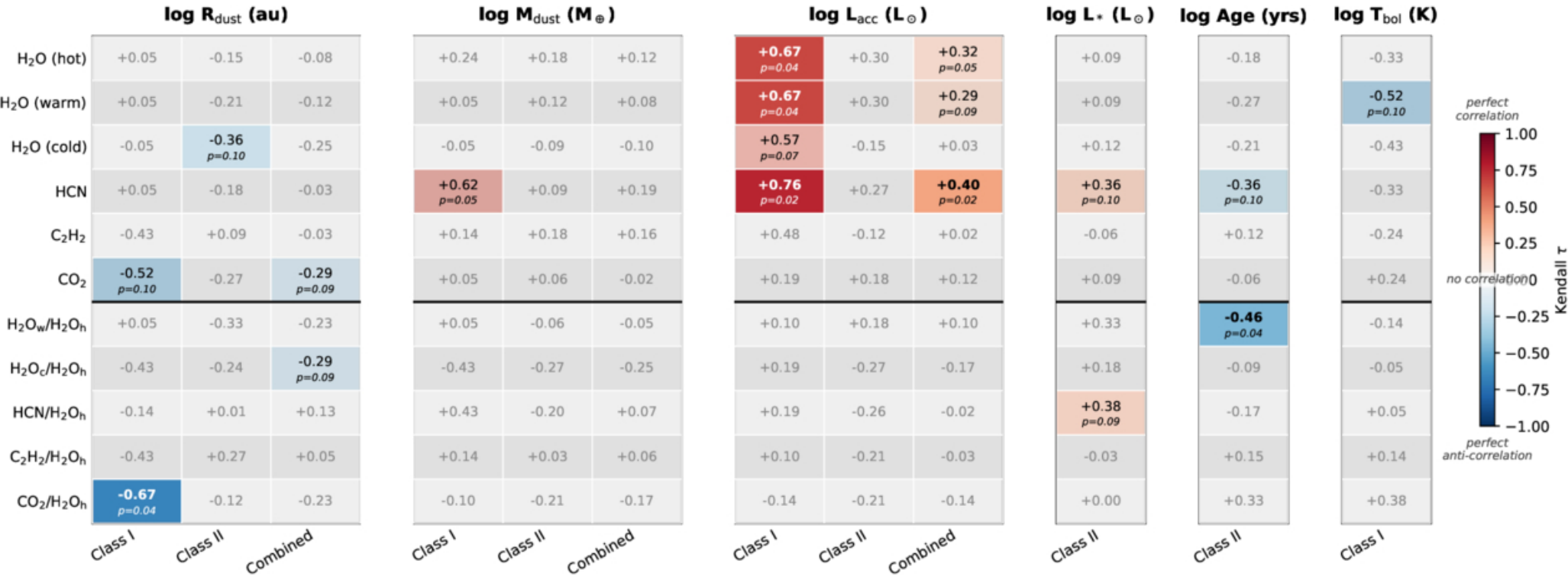
Figure 9. from Ke Zhang et al 2026 Astron. J. 172 doi:10.3847/1538-3881/ae90a1 https://dx.doi.org/10.3847/1538-3881/ae90a1 © 2026. The Author(s). Published by the American Astronomical Society.
