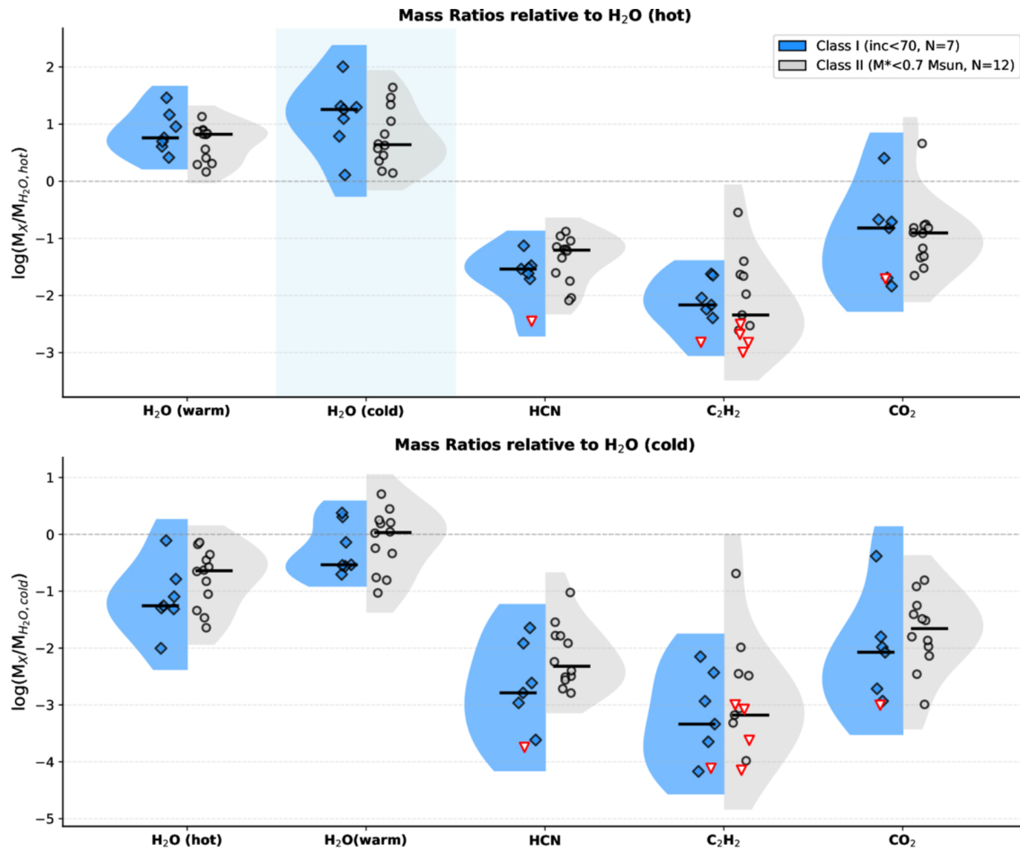
Figure 8. from Ke Zhang et al 2026 Astron. J. 172 doi:10.3847/1538-3881/ae90a1 https://dx.doi.org/10.3847/1538-3881/ae90a1 © 2026. The Author(s). Published by the American Astronomical Society.
